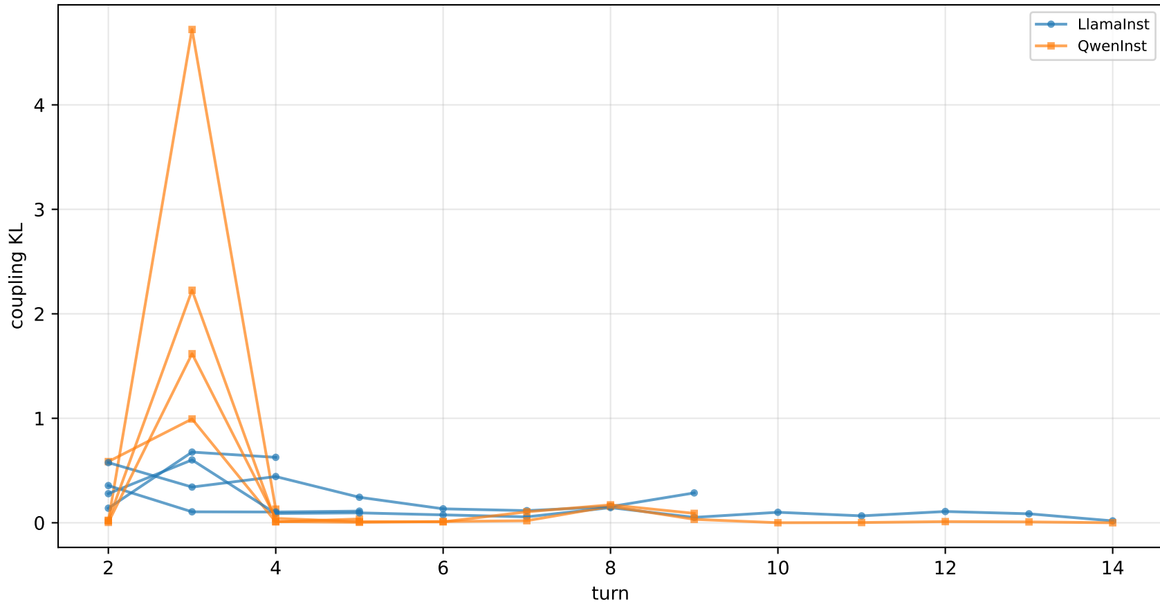
coupling KL every turn, every game (4 games) — game1open_llm_LlamaInst_vs_QwenInst_transcript_coupling_allturns.pdf
