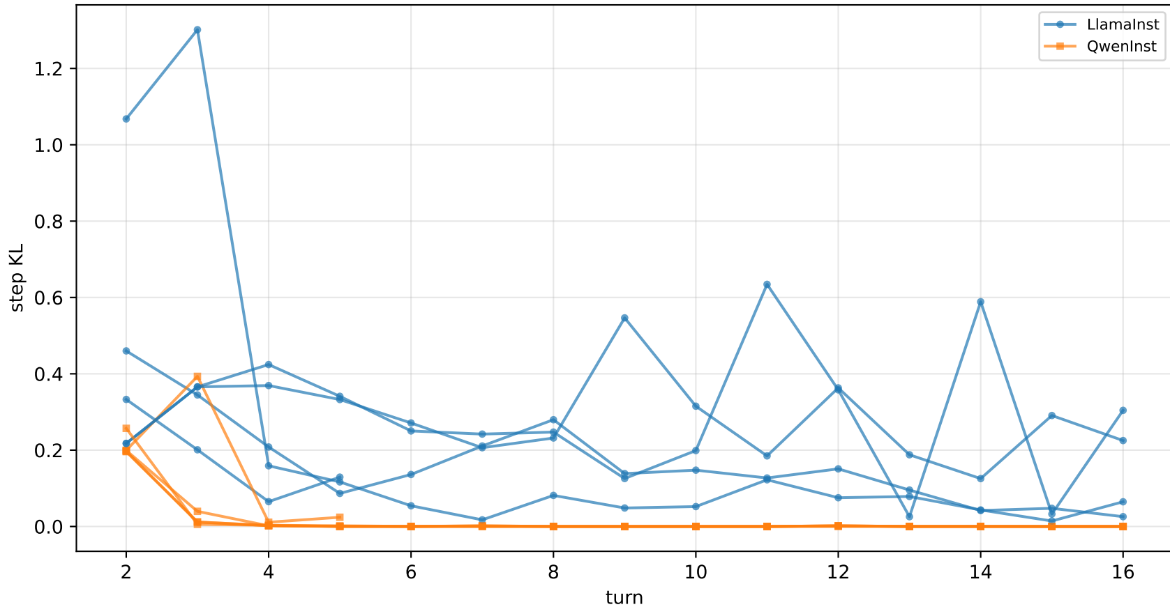
step KL every turn, every game (5 games) — game1sem_llm_LlamaInst_vs_QwenInst_transcript_stepkl_allturns.pdf
