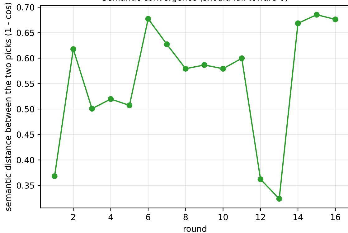
Semantic convergence (should fall toward 0)
