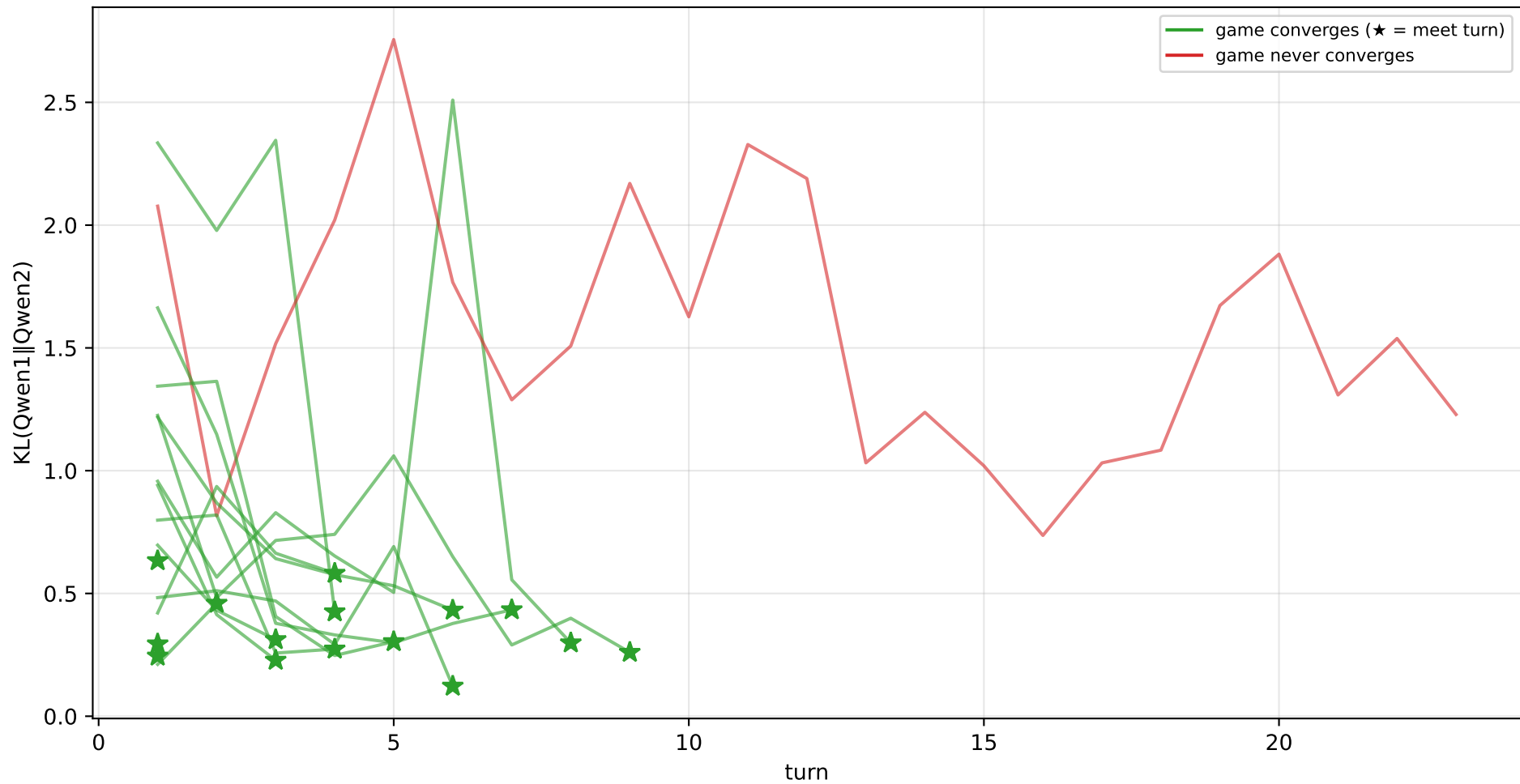
reactive: cross-model KL per turn, all games
