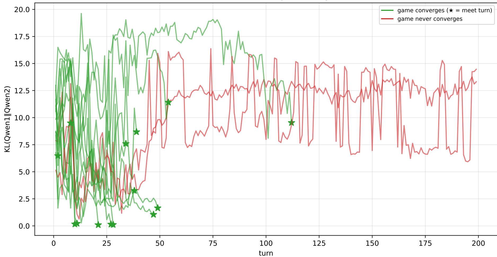
nolist-fruit: cross-model KL per turn, all games
