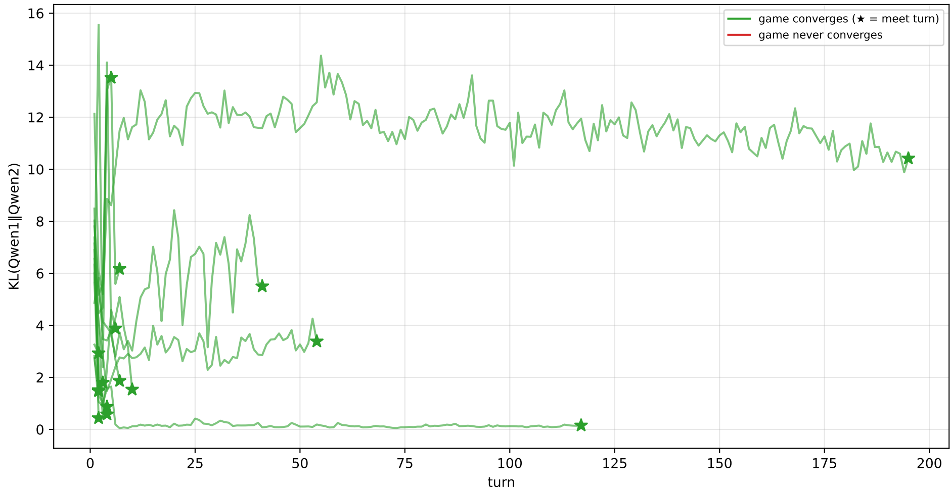
repeatok-fruit: cross-model KL per turn, all games
