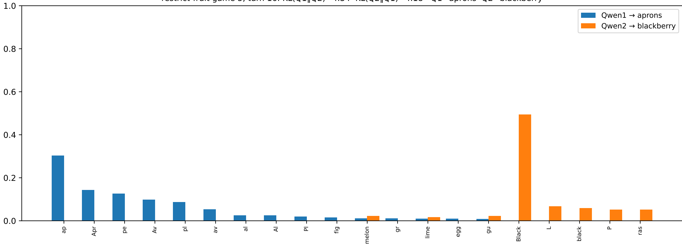
restrict-fruit game 5, turn 16: KL(Q1\|Q2)=4.34 KL(Q2\|Q1)=4.18 Q1=aprons Q2=blackberry
