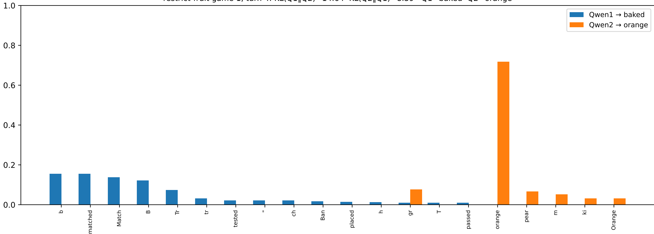
restrict-fruit game 1, turn 4: KL(Q1\|Q2)=14.64 KL(Q2\|Q1)=8.39 Q1=baked Q2=orange
