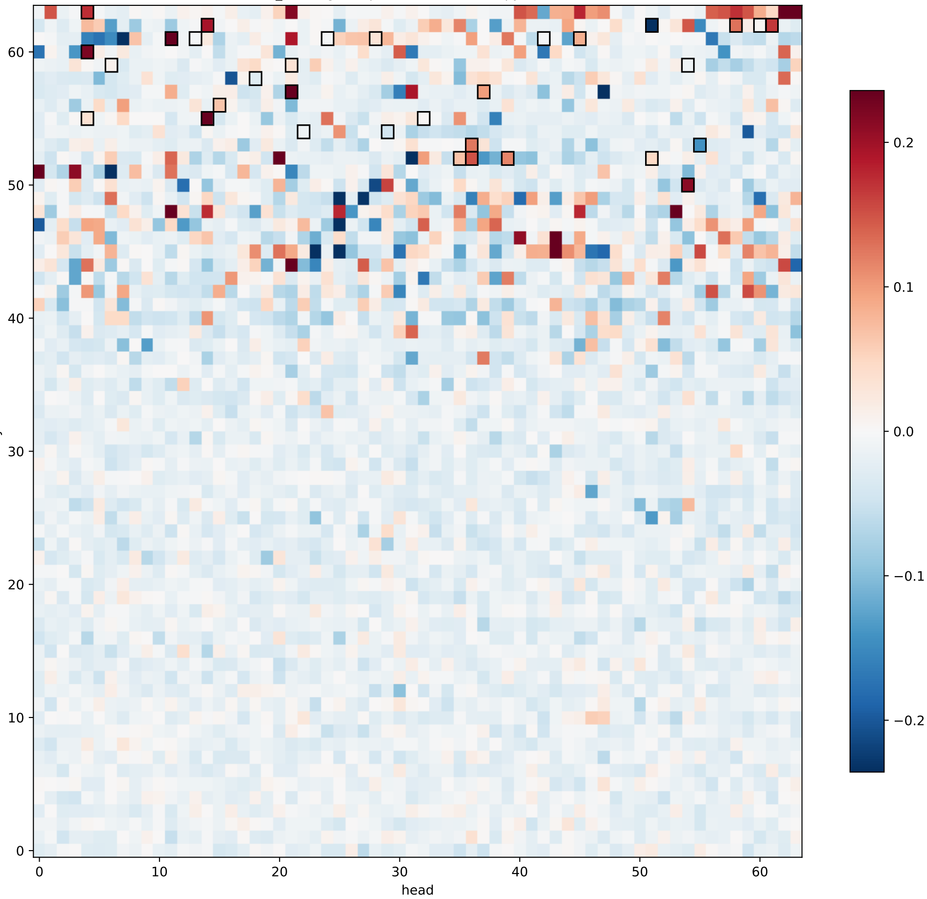
mean d_cue (logit drop of CUE words — copy contribution)
