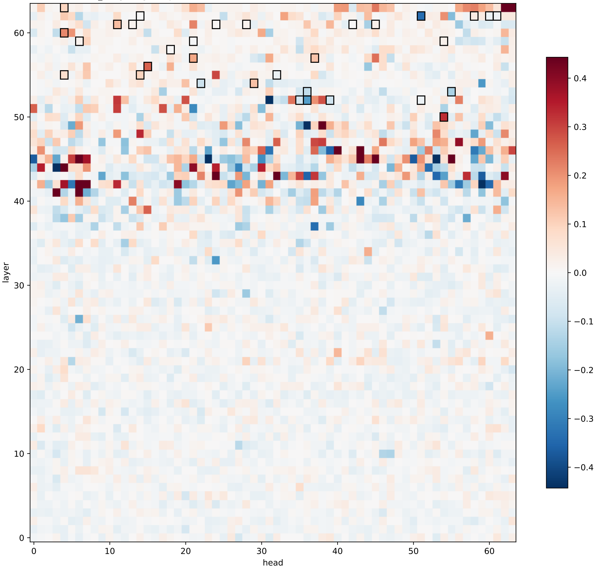
mean d_bridge (logit drop of BRIDGE word when head ablated) — boxes = top-32 restoration heads
