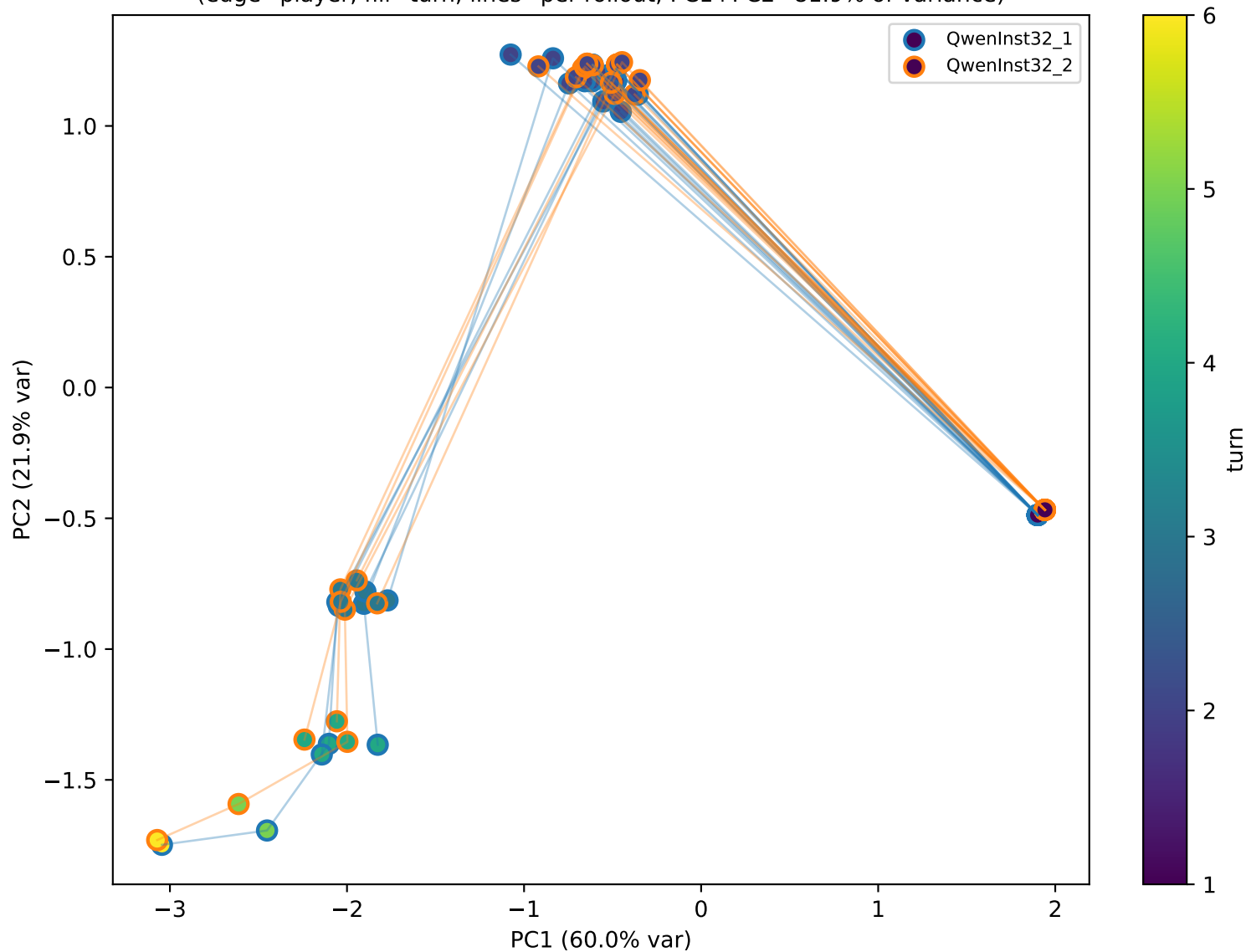
QwenInst32 self-play — residual PCA @ layer 9/64 [global centered] (edge=player, fill=turn; lines=per-rollout; PC1+PC2=81.9% of variance)
