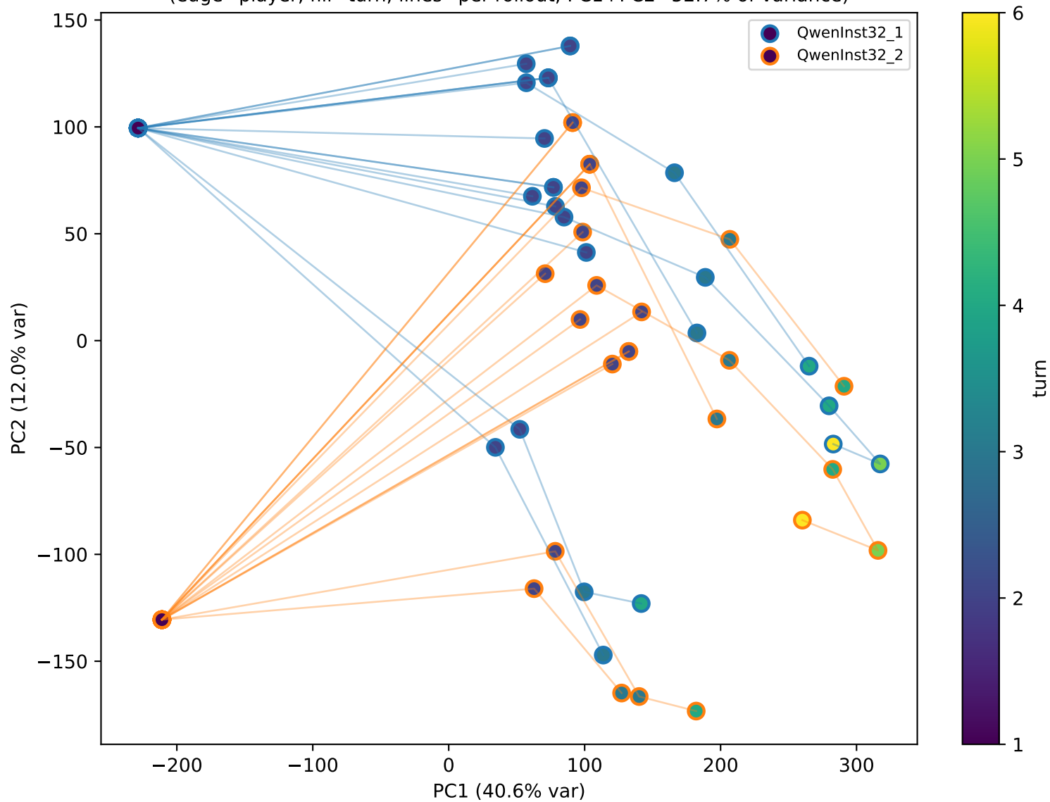
QwenInst32 self-play — residual PCA @ layer 59/64 [global centered] (edge=player, fill=turn; lines=per-rollout; PC1+PC2=52.7% of variance)
