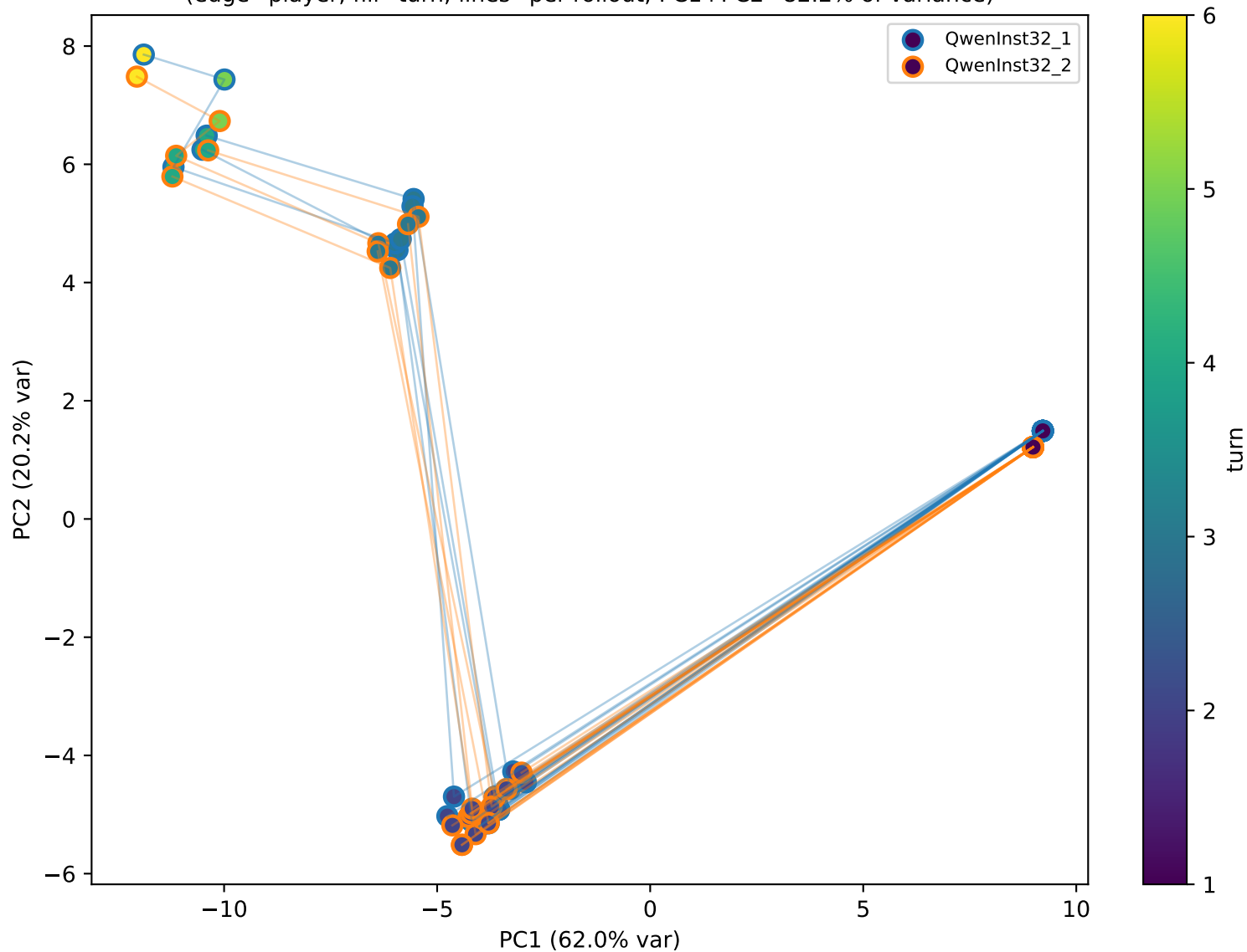
QwenInst32 self-play — residual PCA @ layer 19/64 [global centered] (edge=player, fill=turn; lines=per-rollout; PC1+PC2=82.2% of variance)
