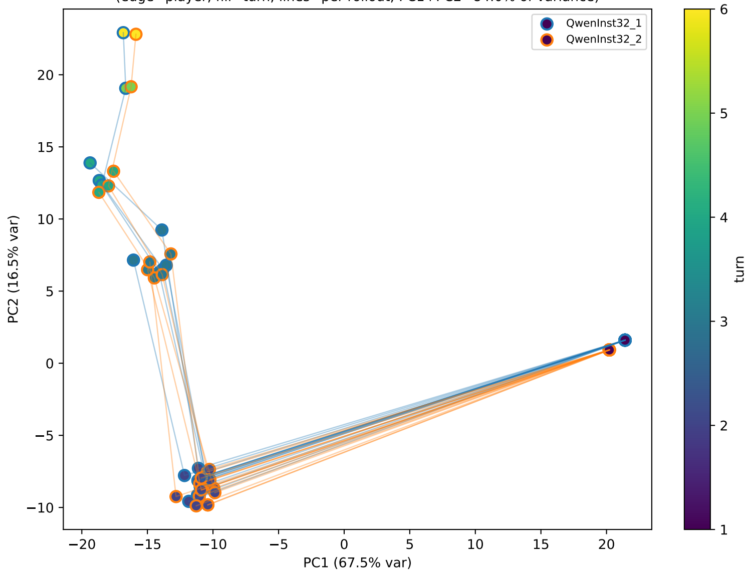
QwenInst32 self-play — residual PCA @ layer 34/64 [global centered] (edge=player, fill=turn; lines=per-rollout; PC1+PC2=84.0% of variance)
