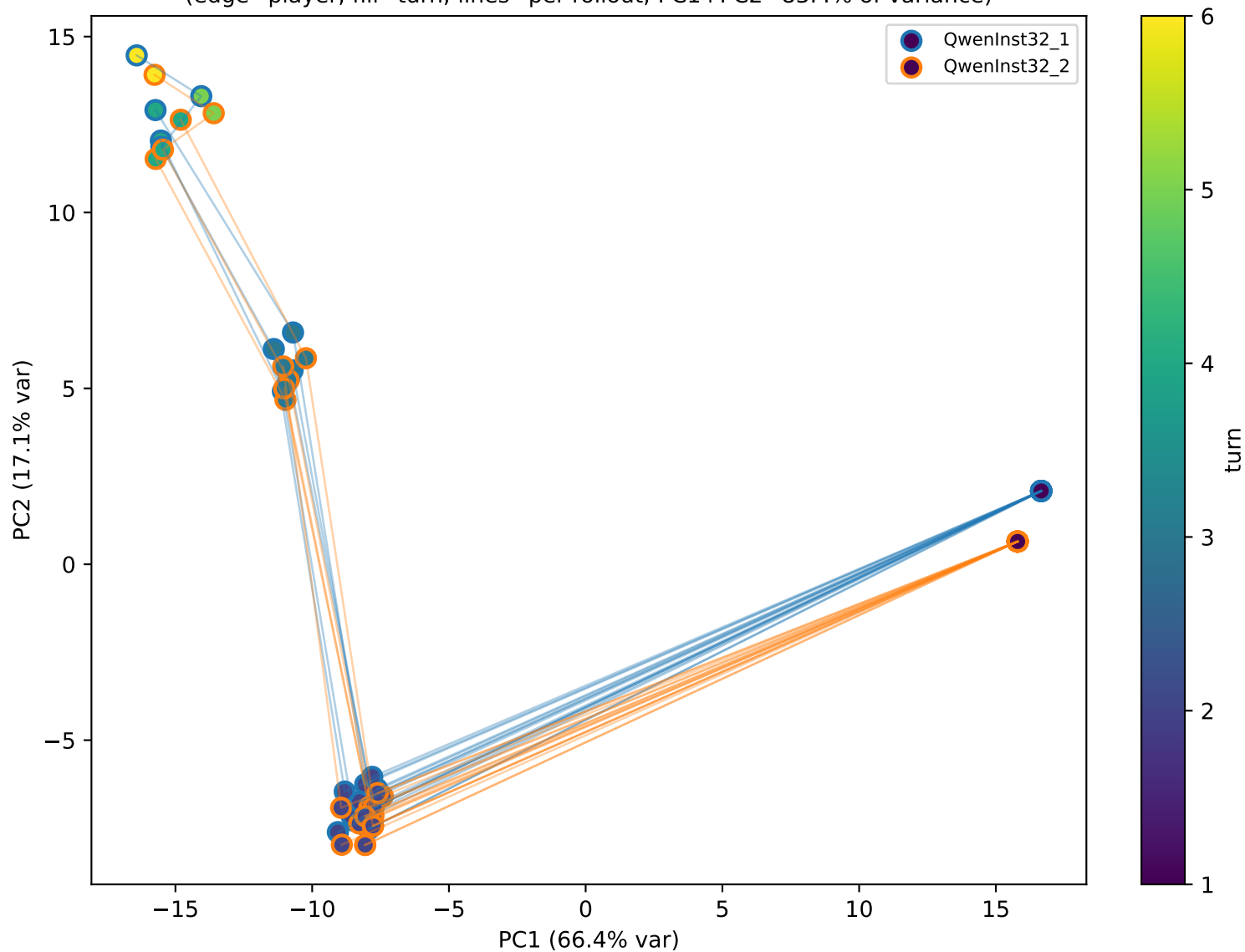
QwenInst32 self-play — residual PCA @ layer 24/64 [global centered] (edge=player, fill=turn; lines=per-rollout; PC1+PC2=83.4% of variance)
