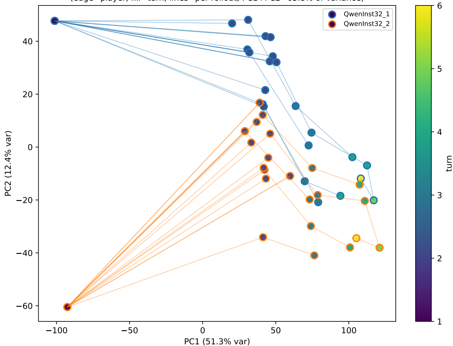
QwenInst32 self-play — residual PCA @ layer 54/64 [global centered] (edge=player, fill=turn; lines=per-rollout; PC1+PC2=63.8% of variance)
