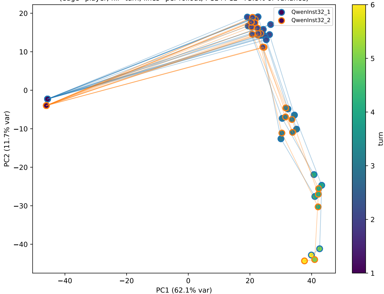
QwenInst32 self-play — residual PCA @ layer 49/64 [global centered] (edge=player, fill=turn; lines=per-rollout; PC1+PC2=73.8% of variance)
