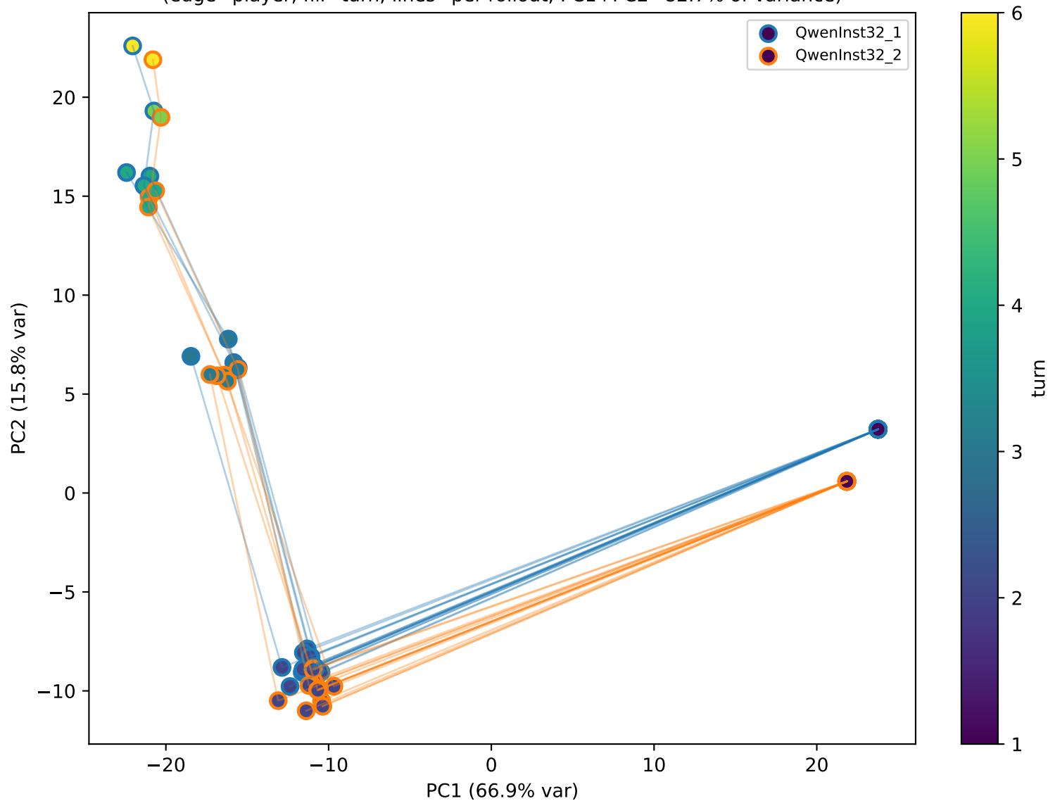
QwenInst32 self-play — residual PCA @ layer 29/64 [global centered] (edge=player, fill=turn; lines=per-rollout; PC1+PC2=82.7% of variance)
