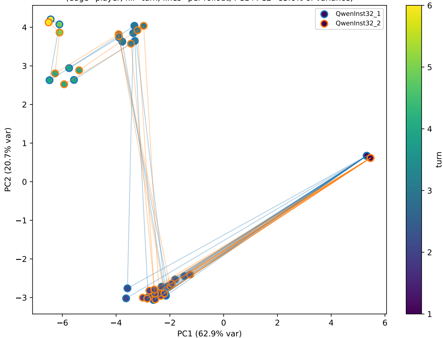
QwenInst32 self-play — residual PCA @ layer 14/64 [global centered] (edge=player, fill=turn; lines=per-rollout; PC1+PC2=83.6% of variance)
