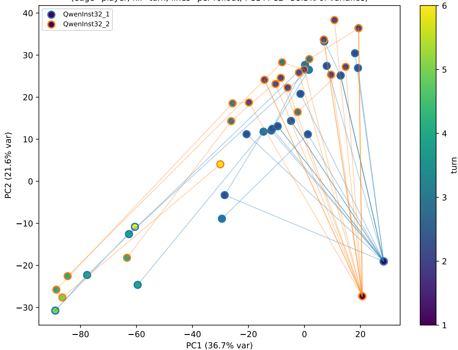
QwenInst32 self-play — residual PCA @ layer 64/64 [global centered] (edge=player, fill=turn; lines=per-rollout; PC1+PC2=58.3% of variance)
