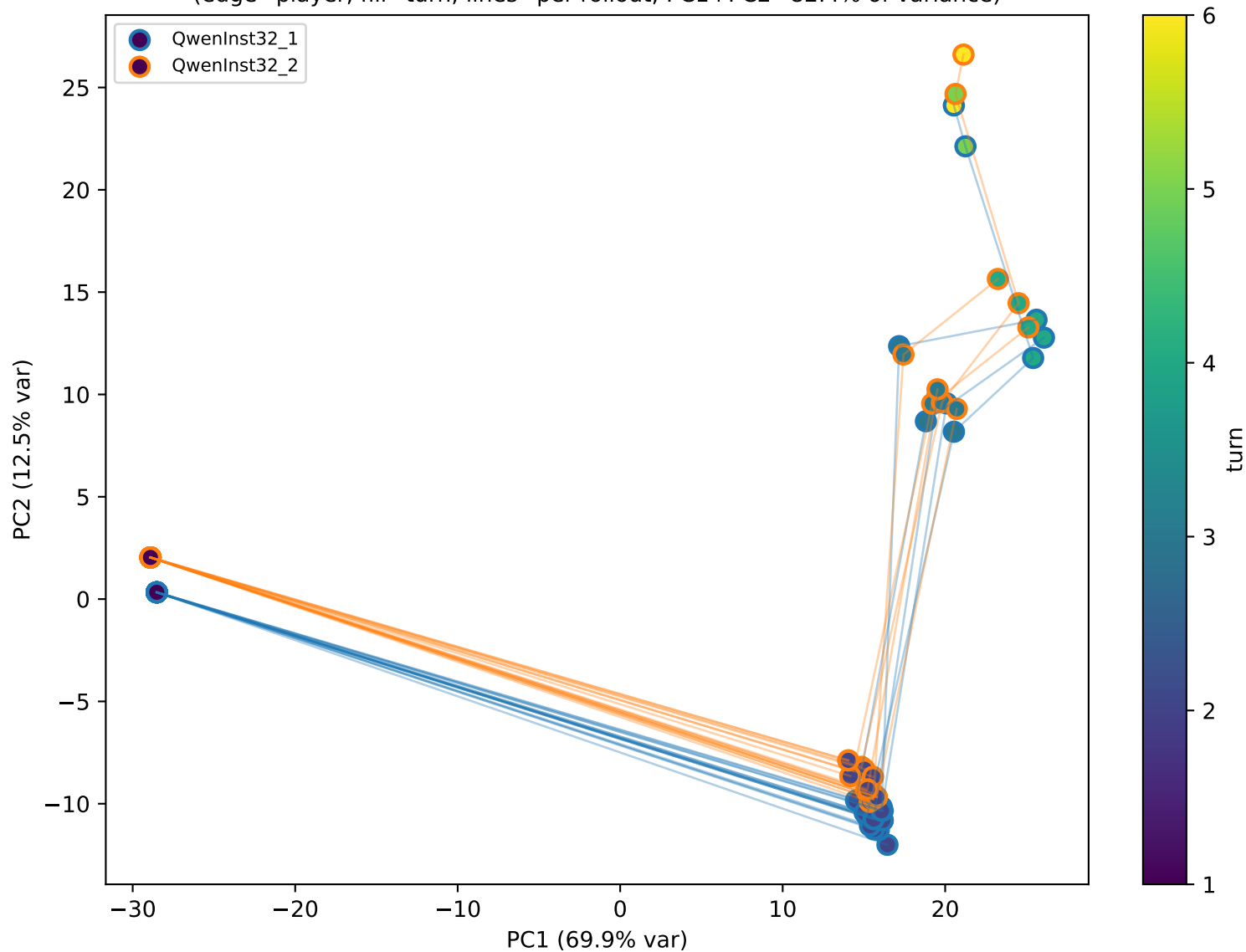
QwenInst32 self-play — residual PCA @ layer 44/64 [global centered] (edge=player, fill=turn; lines=per-rollout; PC1+PC2=82.4% of variance)
