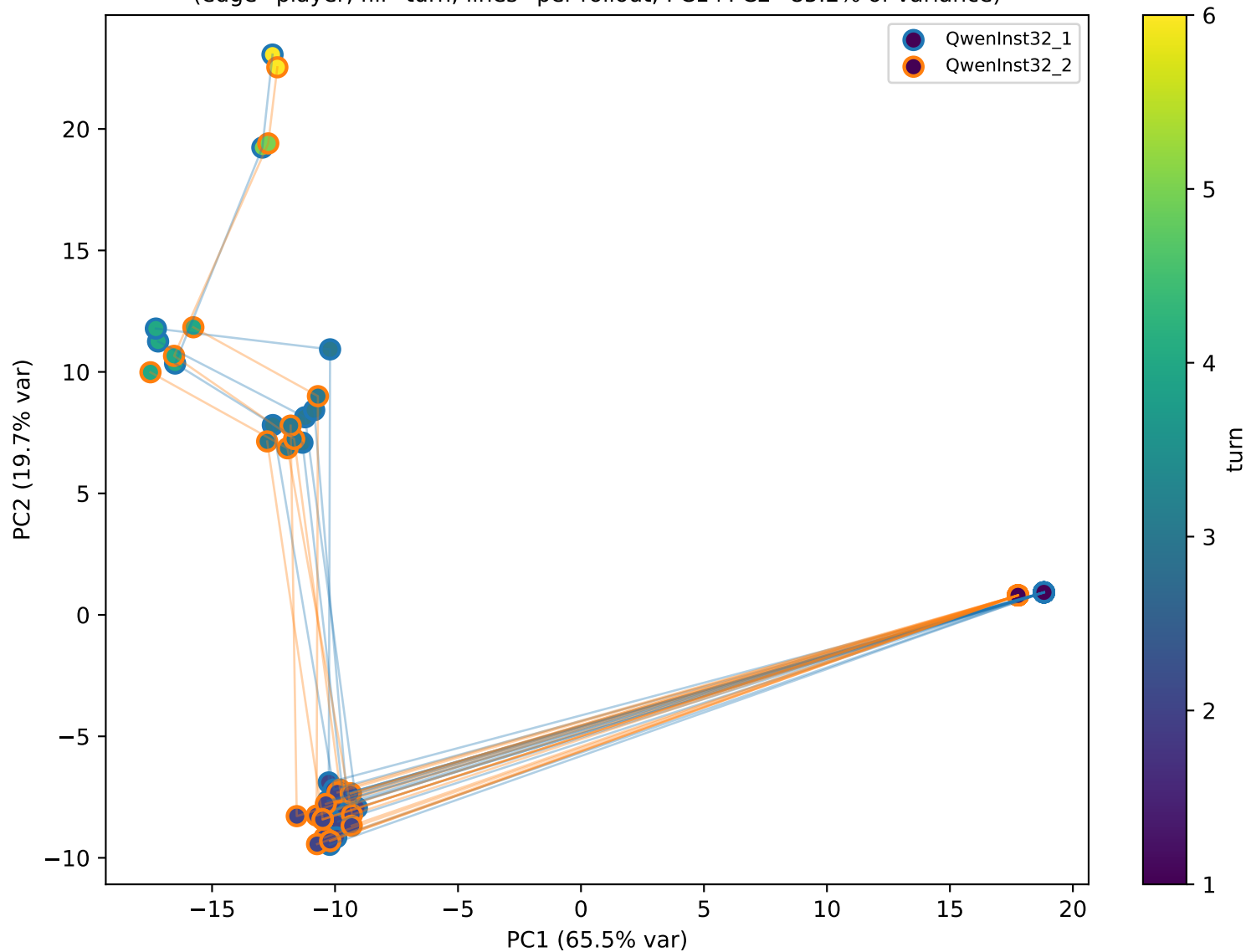
QwenInst32 self-play — residual PCA @ layer 39/64 [global centered] (edge=player, fill=turn; lines=per-rollout; PC1+PC2=85.2% of variance)
