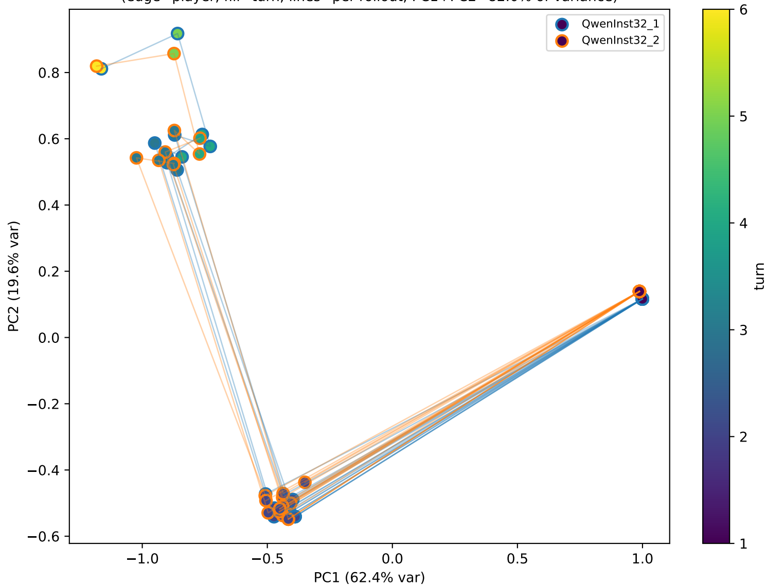
QwenInst32 self-play — residual PCA @ layer 4/64 [global centered] (edge=player, fill=turn; lines=per-rollout; PC1+PC2=82.0% of variance)
