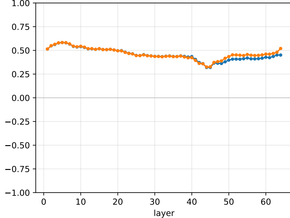
corr(convergence coordinate, turn)
