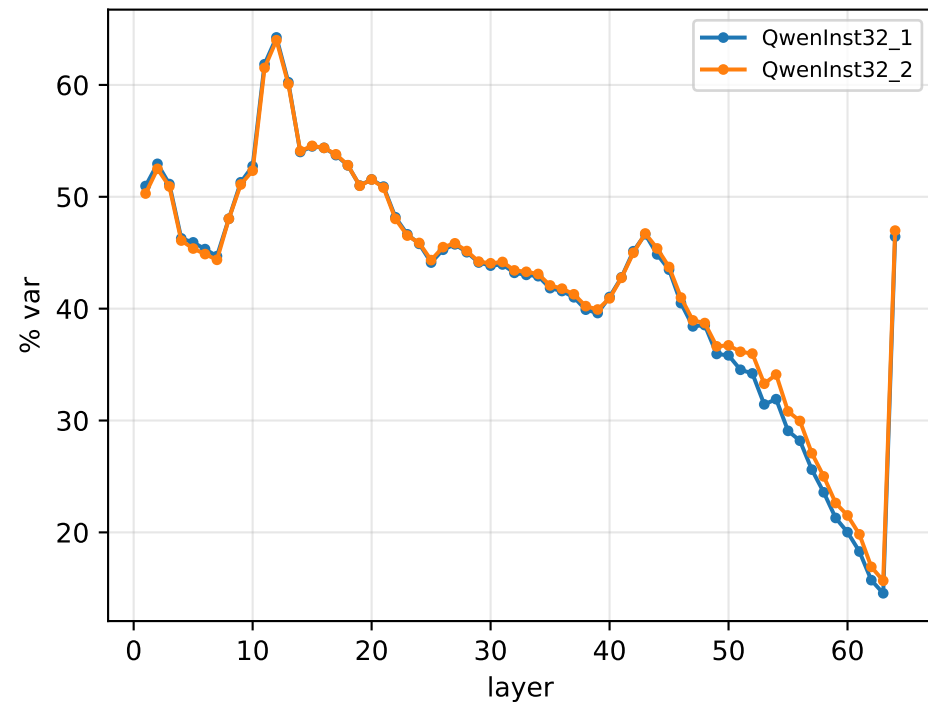
PC1 (convergence dir) % of within-seed variance
