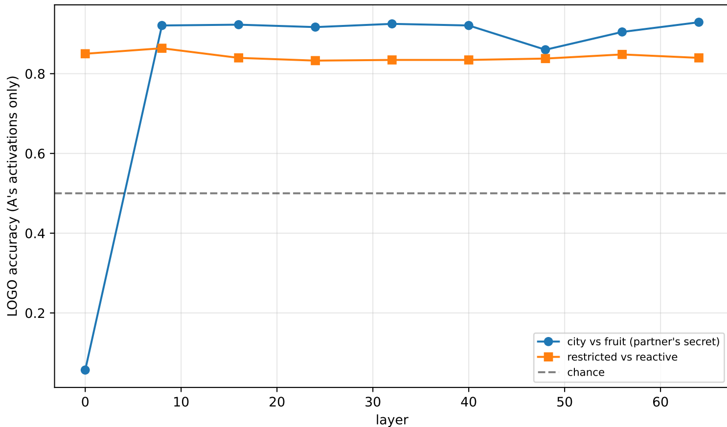
Does the UNRESTRICTED player encode its partner's hidden constraint?
