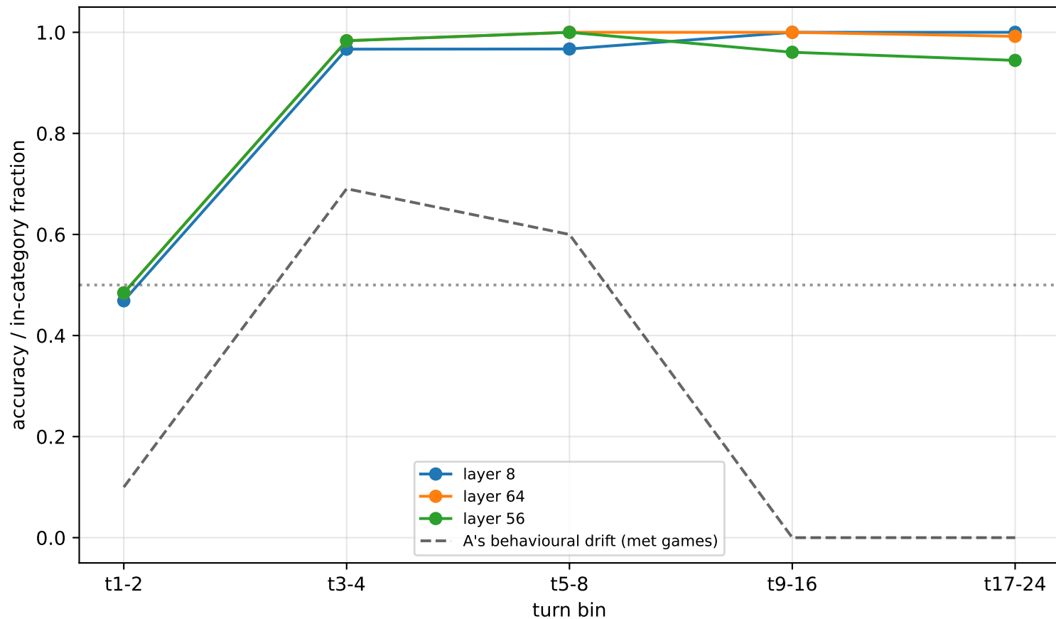
Decoding time-course vs behavioural drift — is the constraint known before behaviour moves?
