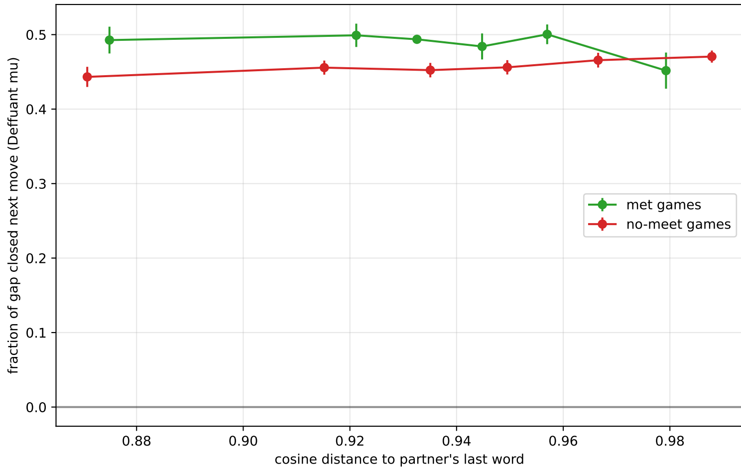
Bounded-confidence test: assimilation vs distance Deffuant predicts \mu > 0 near, \sim 0 far (threshold)
