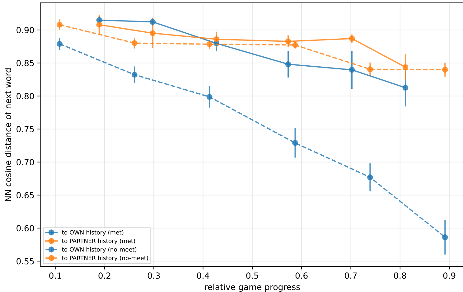
Urn test: does the walk cling to its own neighborhood? (solid=met, dashed=no-meet)
