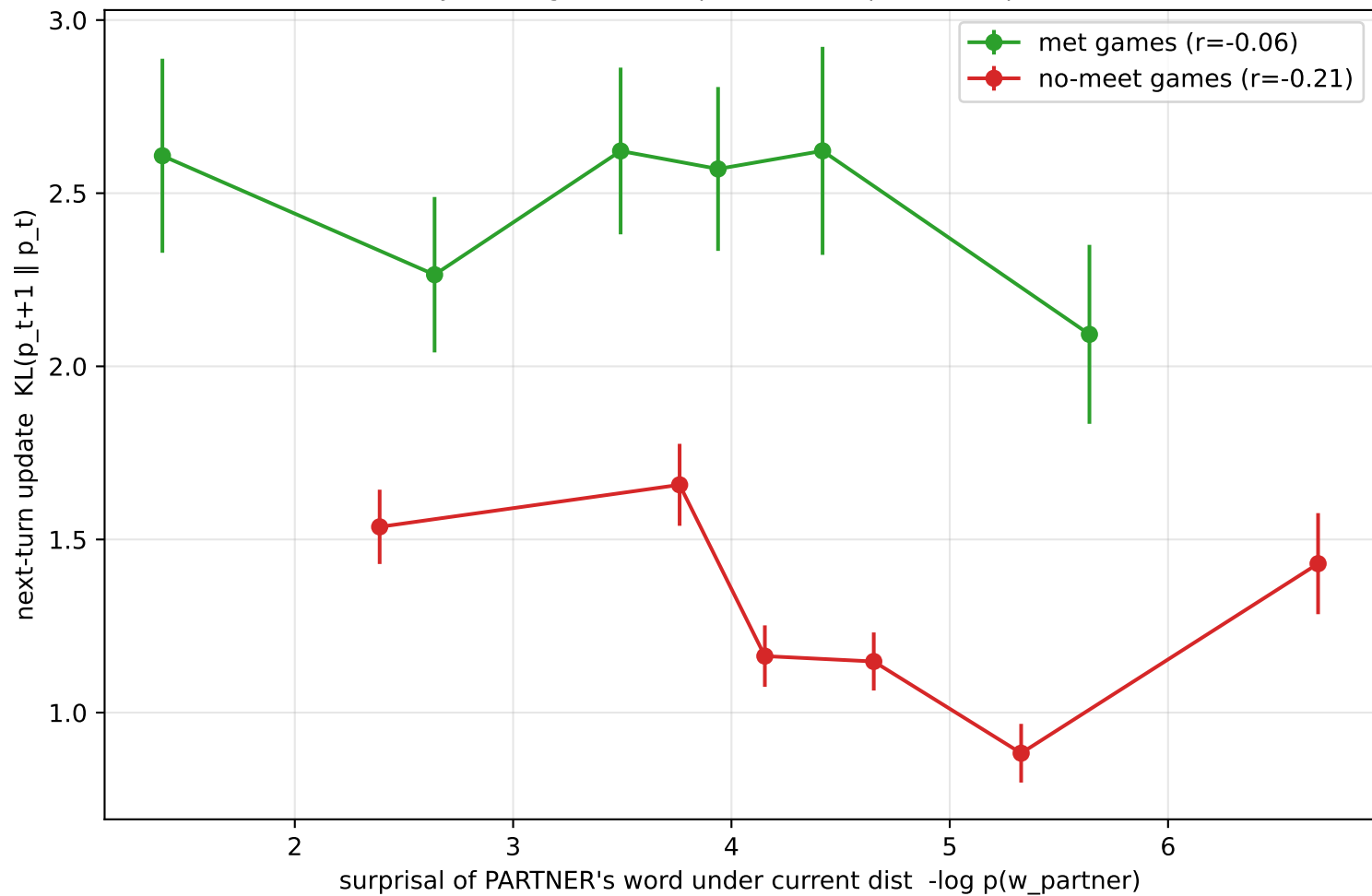
Bayesian signature 1: update size vs partner surprisal
