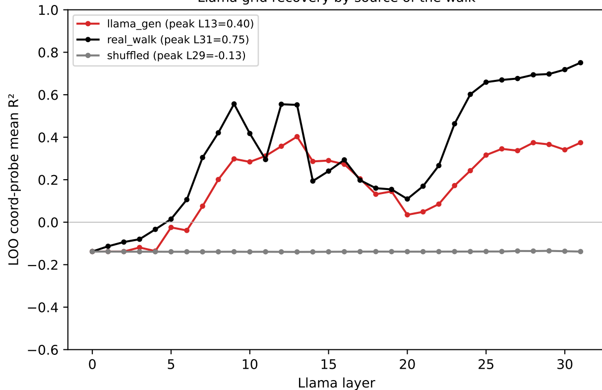
Llama grid recovery by source of the walk
