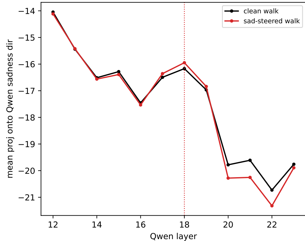
Qwen sadness projection over the walk
