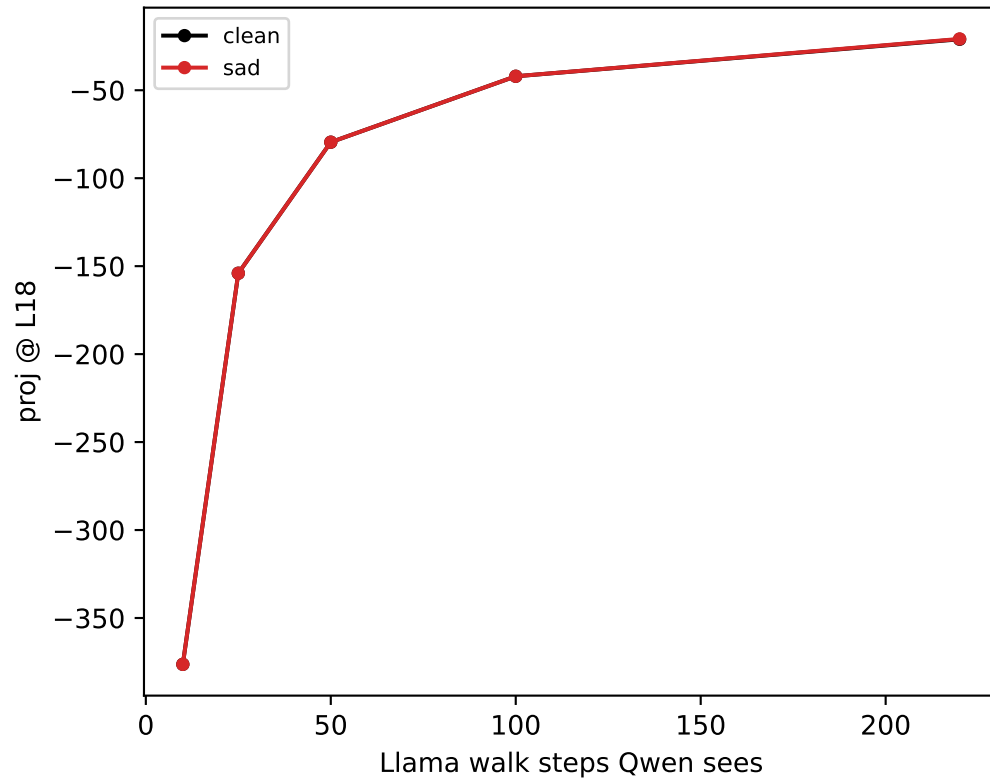
Sadness vs context length
