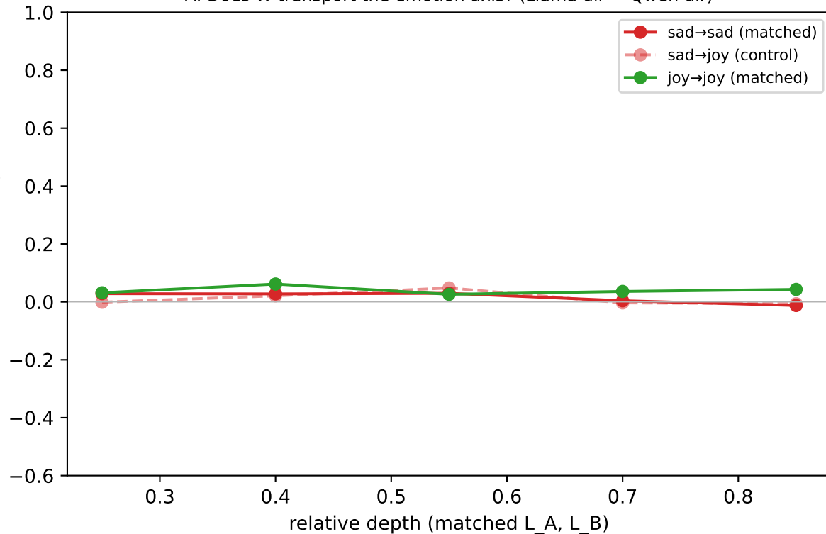
A. Does W transport the emotion axis? (Llama dir \rightarrow Qwen dir)
