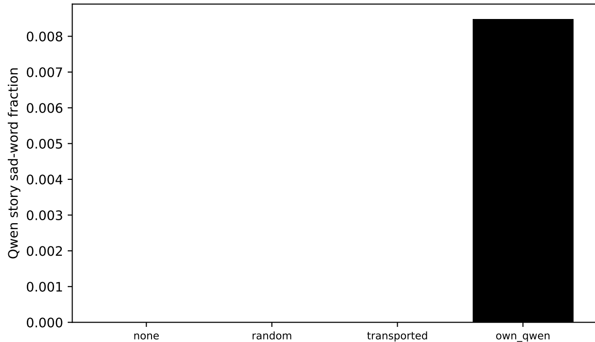
B. Steer Qwen@L20 with transported sad dir (cos vs own-Qwen sad=+0.03)
