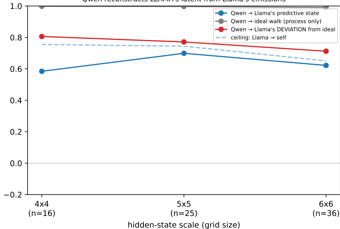
Qwen reconstructs LLAMA's latent from Llama's emissions
