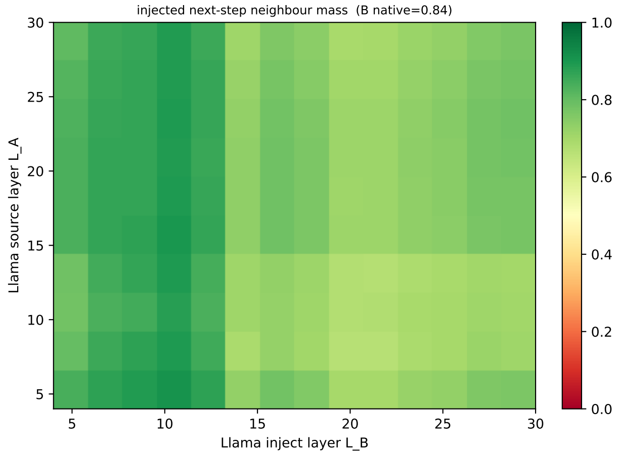
[square_grid] Llama→Llama: alignment R^2 (left) vs injected behaviour (right) over L_A \times L_B
