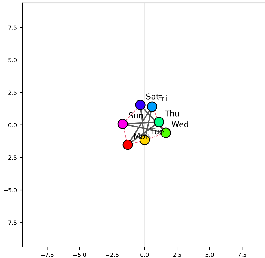
PRETRAINED plane (fixed) — 2.8% of variance
