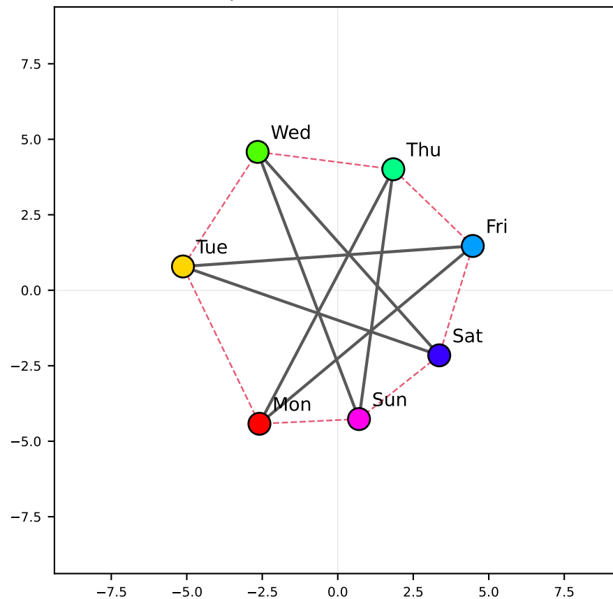
FINAL learned plane (fixed) — 38.9% of variance
