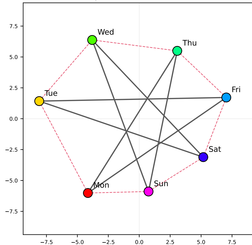
FINAL learned plane (fixed) — 55.2% of variance
