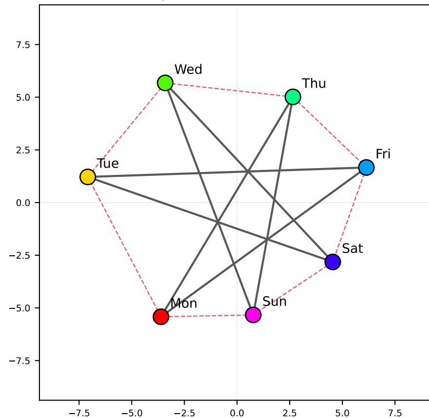
FINAL learned plane (fixed) — 50.7% of variance
