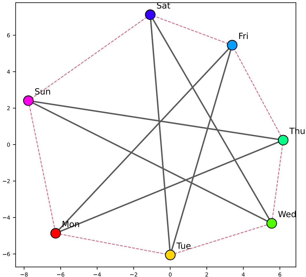
PRETRAINED weekday ring (neutral templates, no walk) layer 26 — solid: in-context edges, dashed: semantic edges
