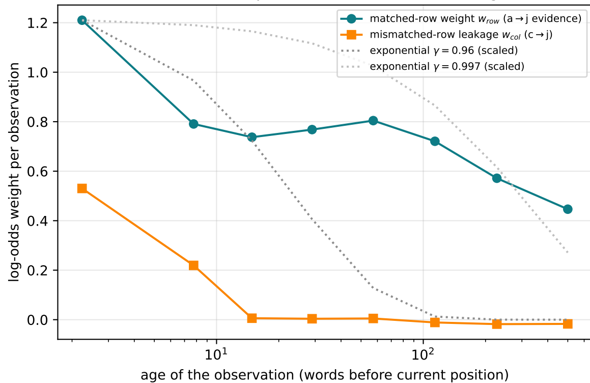
measured in-context update kernel (Llama-3.1-8B, grid walks)
