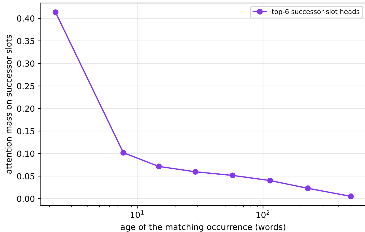
mechanism: induction-head attention by evidence age
