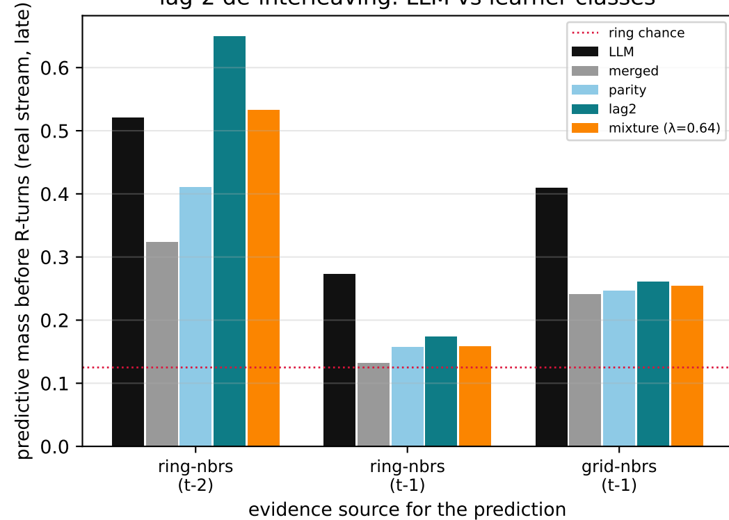
lag-2 de-interleaving: LLM vs learner classes
