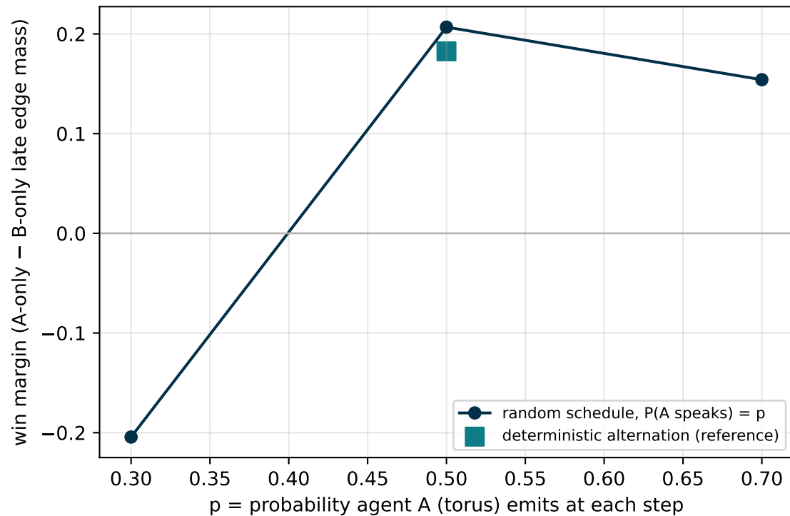
(6a) speaking share sets influence: the 30% speaker loses
