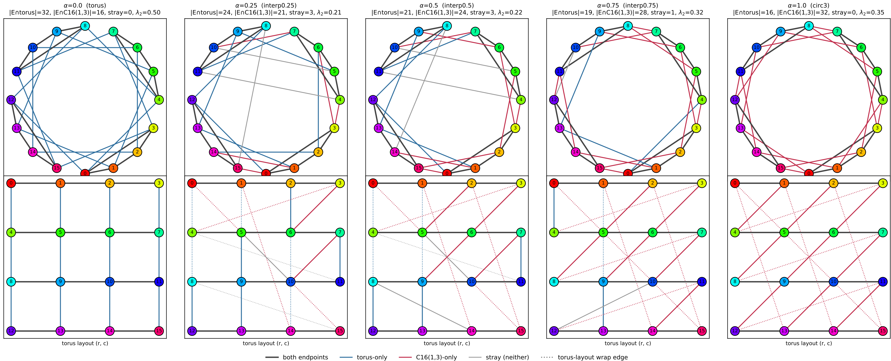
Ground-truth interpolation family G_\alpha : degree-preserving swaps from torus C4 \times C4 ( \alpha=0 ) to circulant C16(\pm 1, \pm 3) ( \alpha=1 ); all 16 nodes, 4-regular, 32 edges
