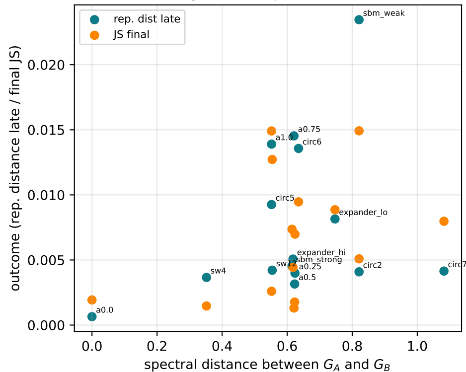
convergence vs spectral distance
