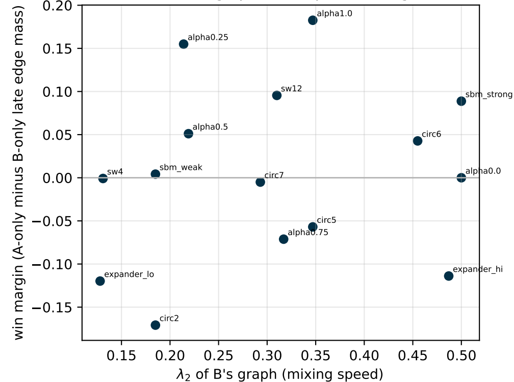
does mixing speed set prior strength?
