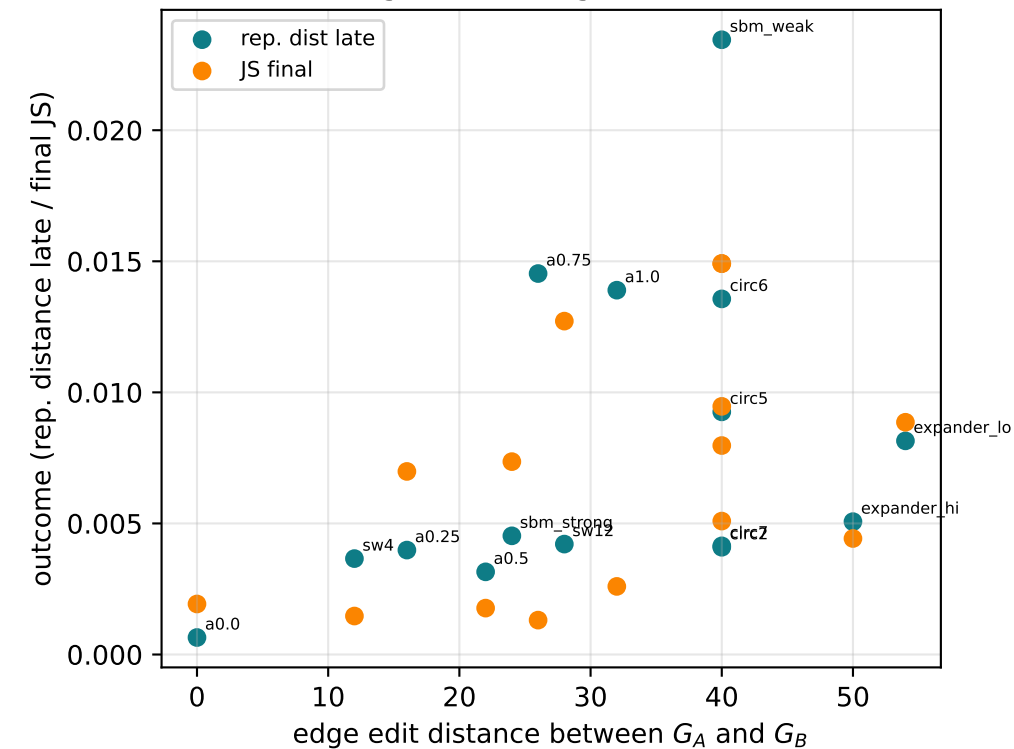
convergence vs edge edit distance
