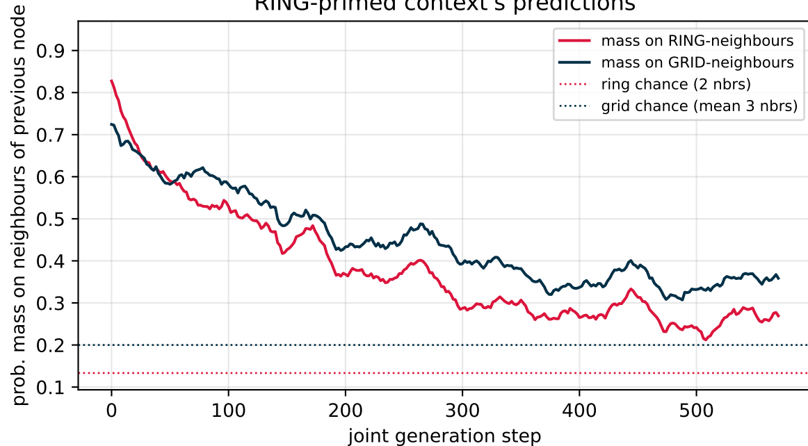
RING-primed context's predictions
