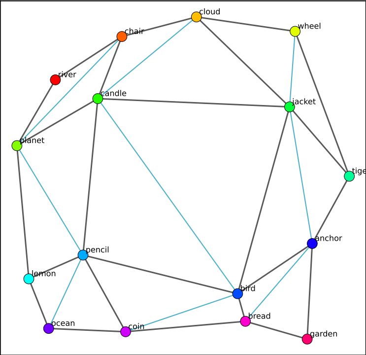
grid-primed | joint_early
