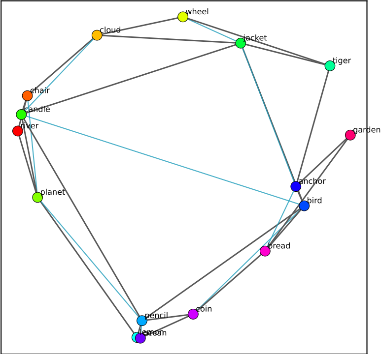
grid-primed | joint_late
