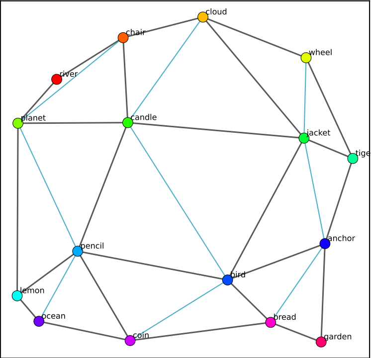
grid-primed | base
