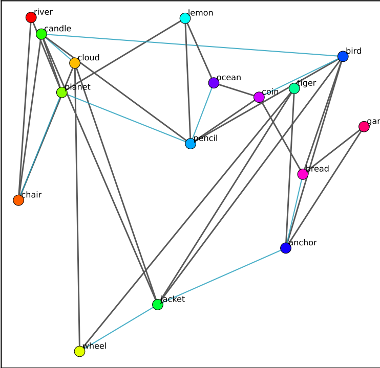
grid-primed | joint_mid
