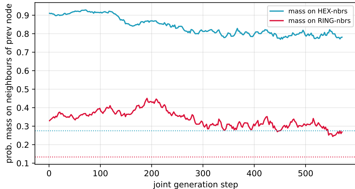
HEX-primed context's predictions
