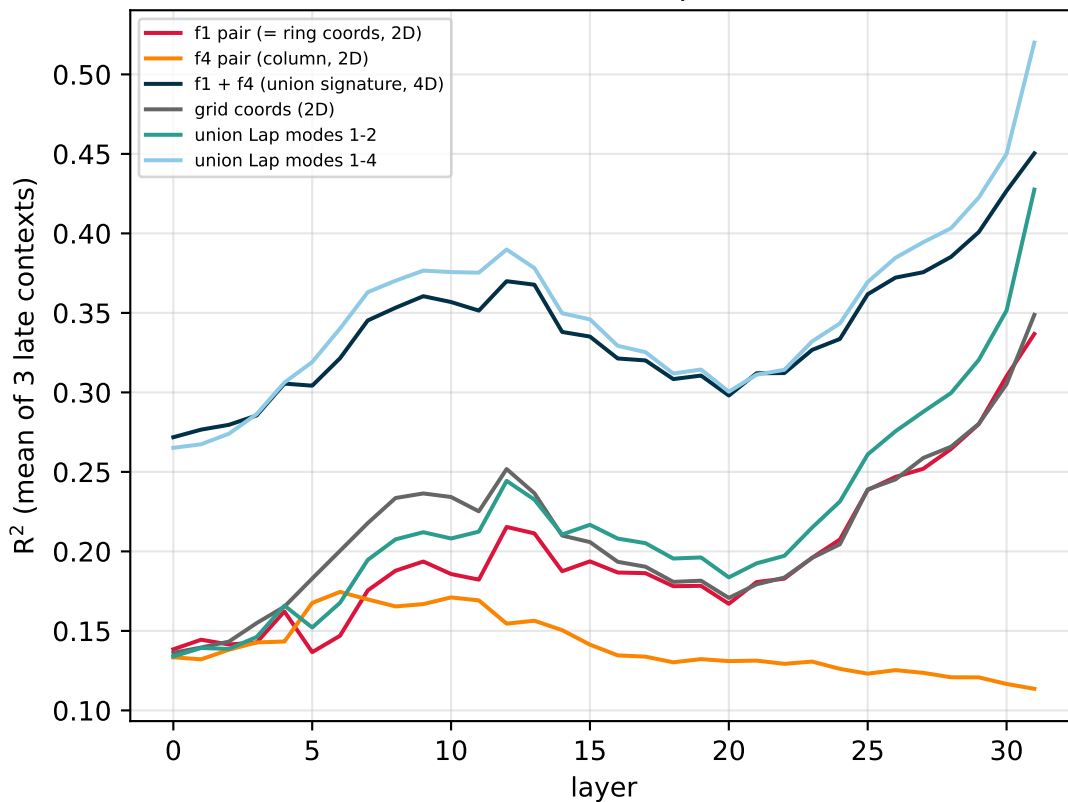
candidate subspaces
