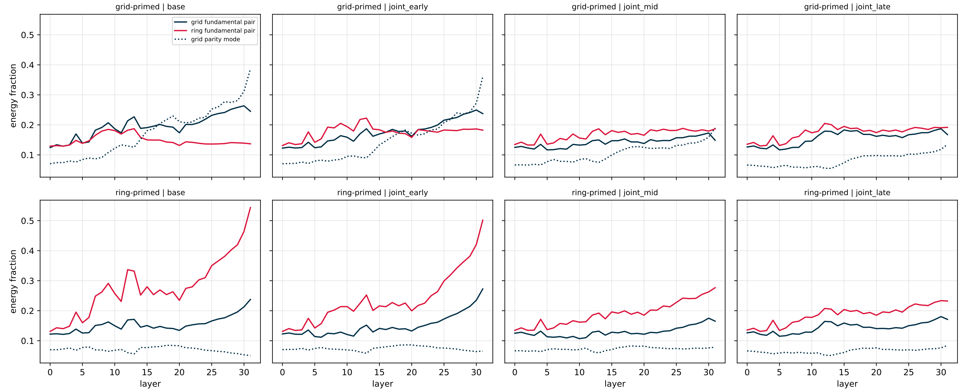
Low-frequency Laplacian eigenmode energy of node-means (grid basis vs ring basis)
