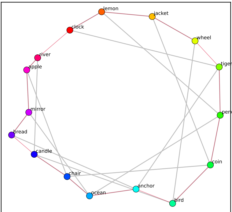
ring-primed | pre-interaction (ctx 700-1000) EVR(2)=0.37
