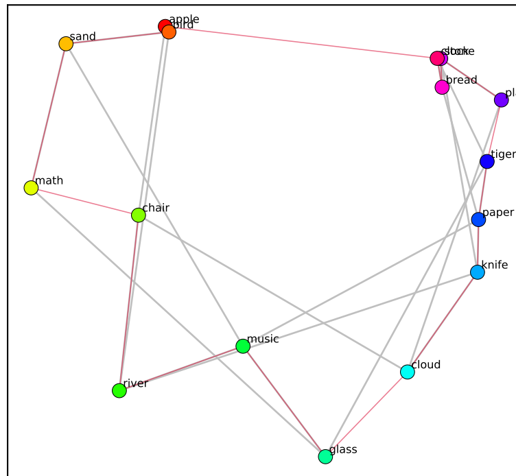
ring-primed | joint steps 0-100 EVR(2)=0.32
