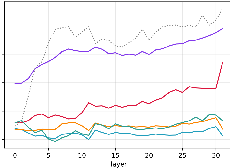
RING-primed late
