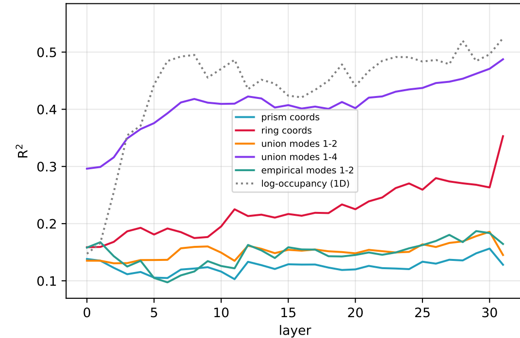
PRISM-primed late
