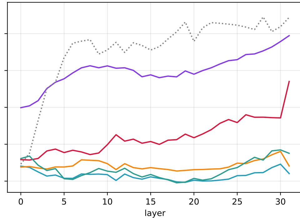
FRESH late
