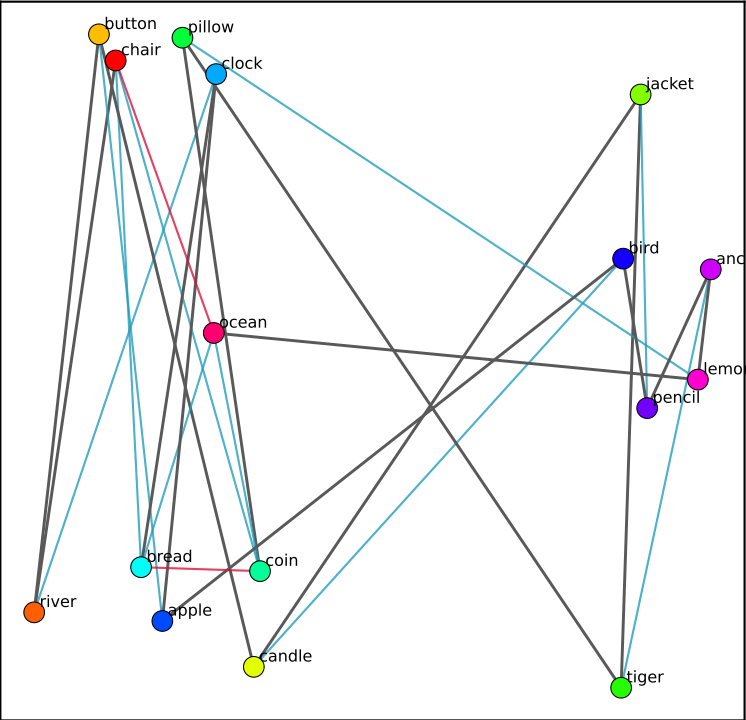
ring-primed | joint_mid
