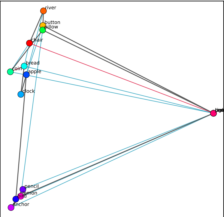
ring-primed | joint_late
