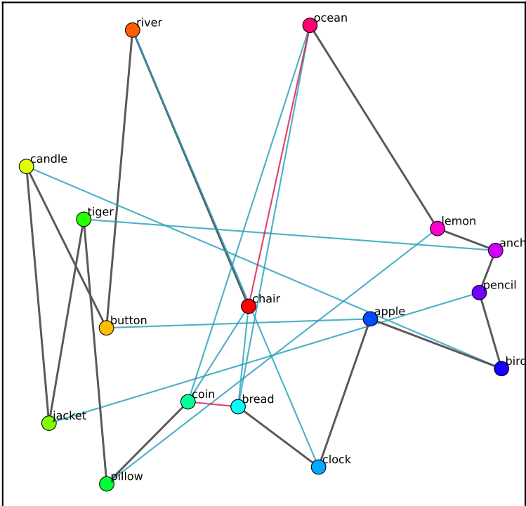
ring-primed | base
