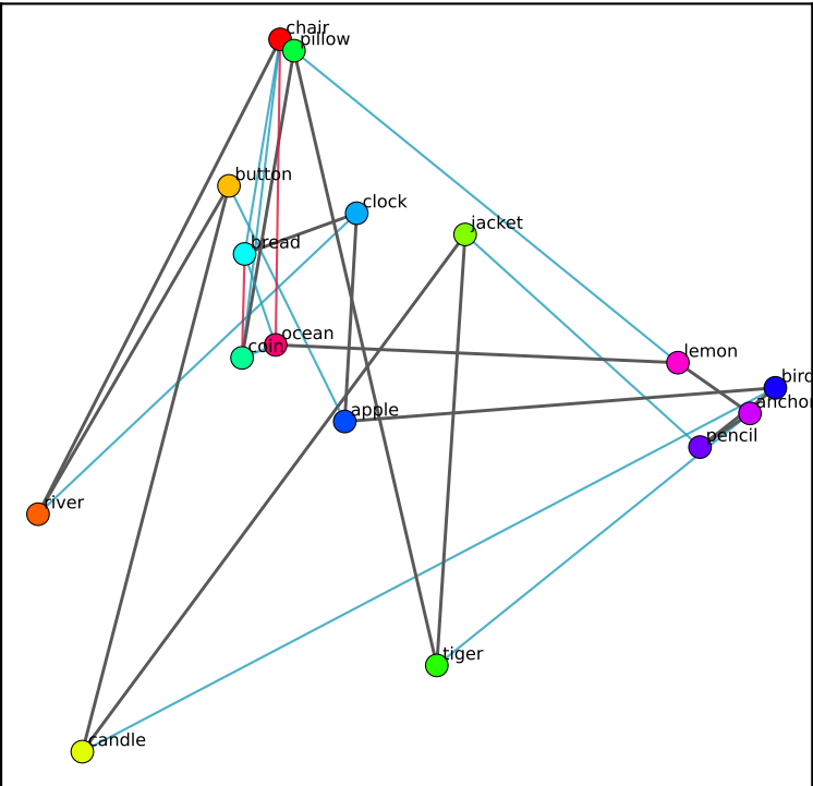
ring-primed | joint_early
