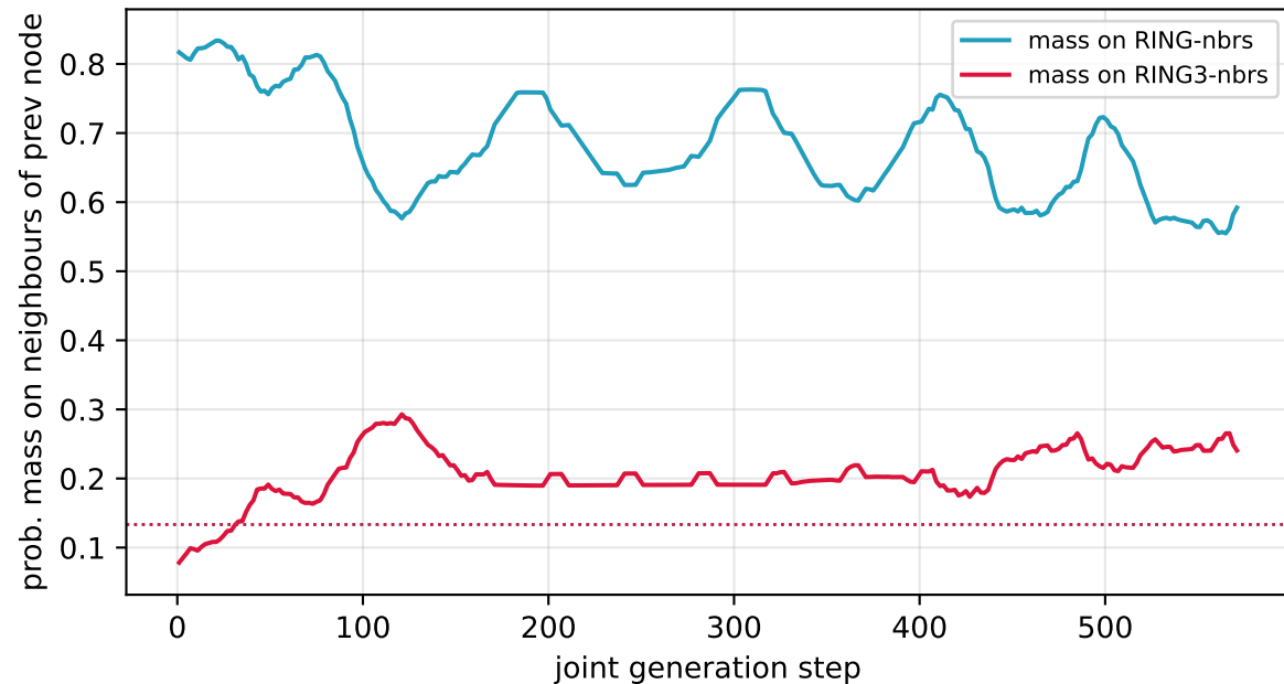
RING-primed context's predictions
