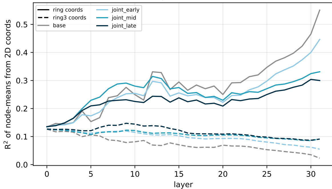
RING-primed context
