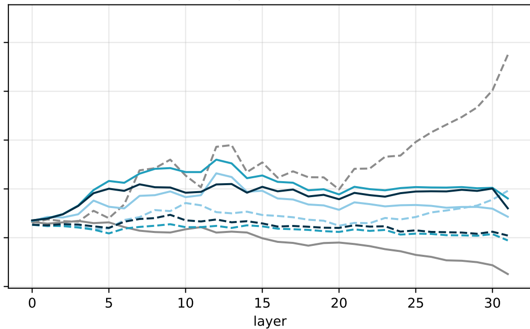
RING3-primed context
