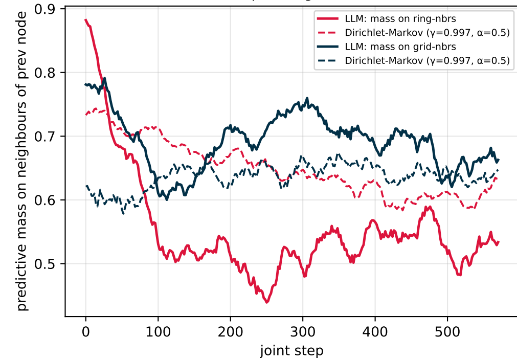
RING-primed generator
