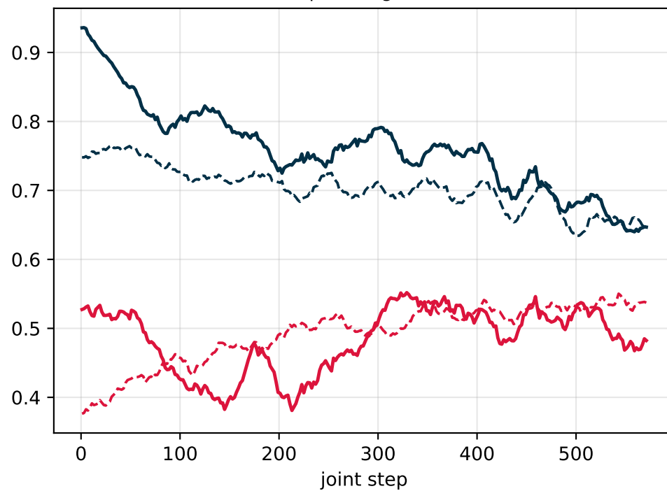
GRID-primed generator
