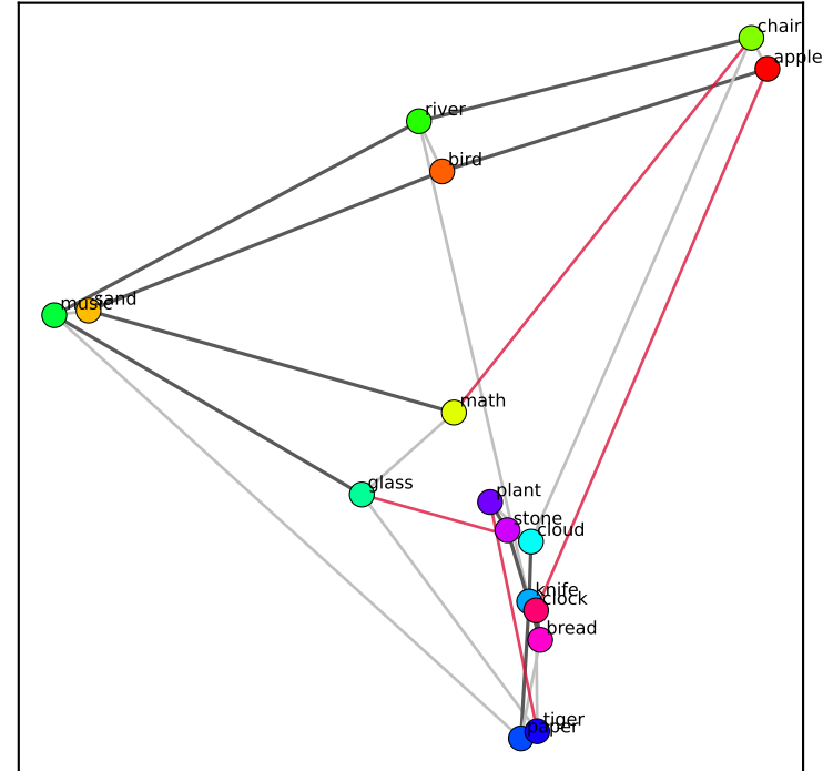
EMPIRICAL stream graph modes 1-2 (aligned)
