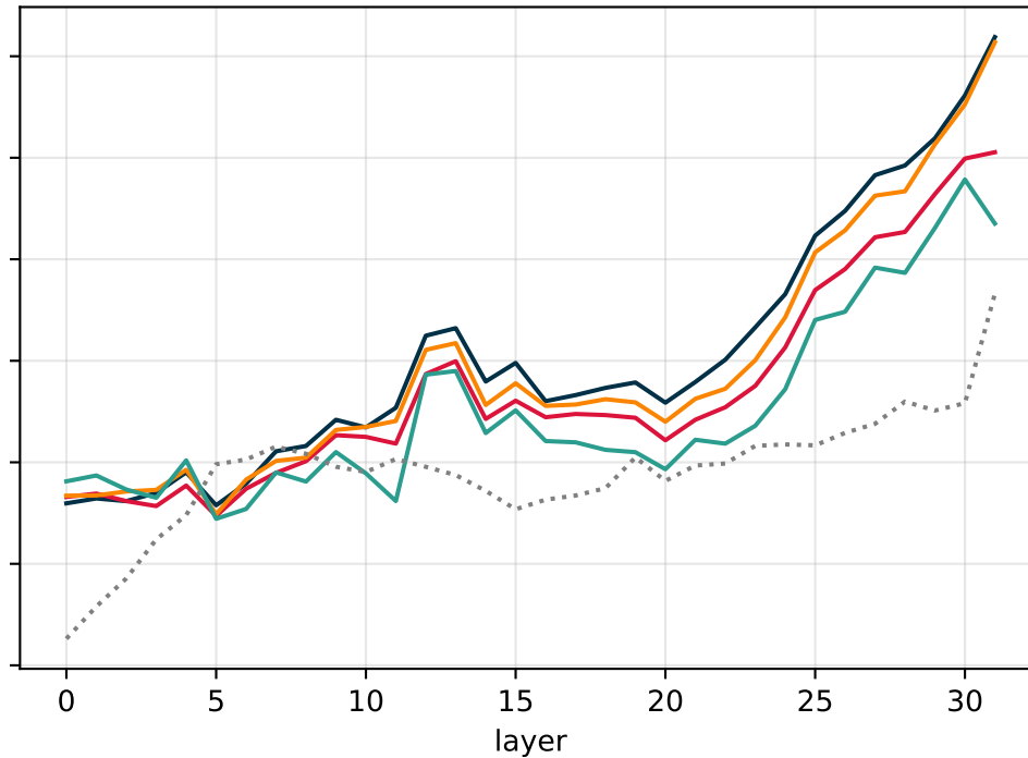
RING-primed, joint_late
