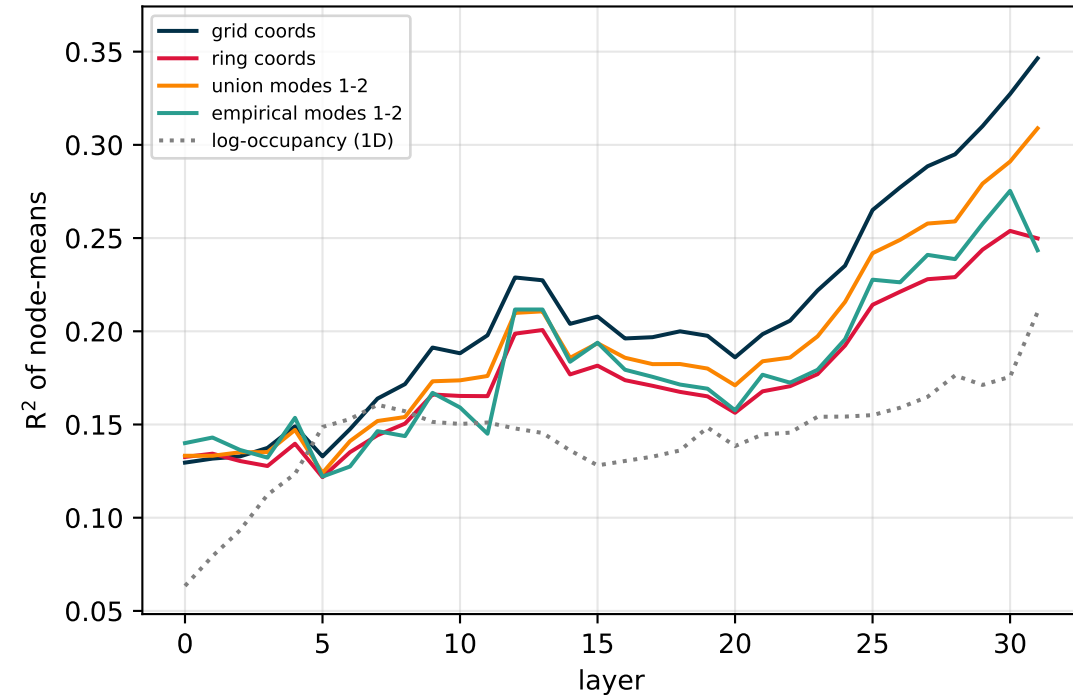
GRID-primed, joint_late
