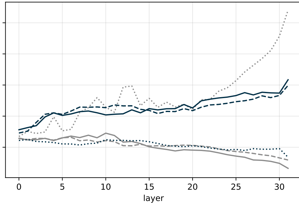
RING3-primed context
