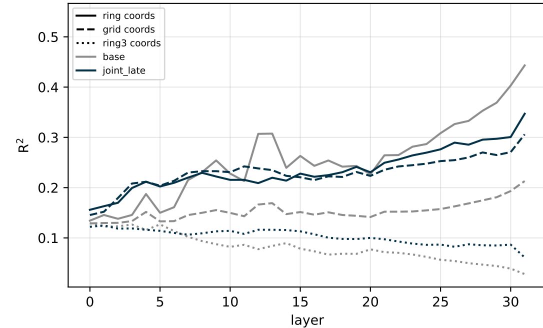
RING-primed context
