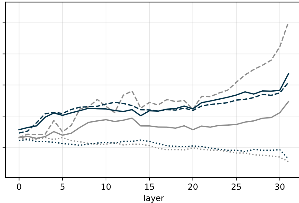
GRID-primed context
