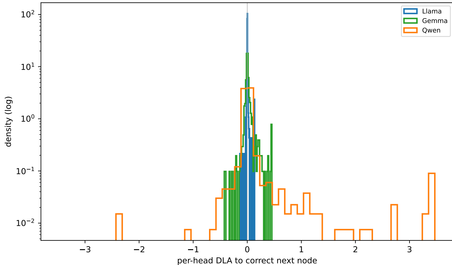
DLA distributions, overlaid (density, log y)
