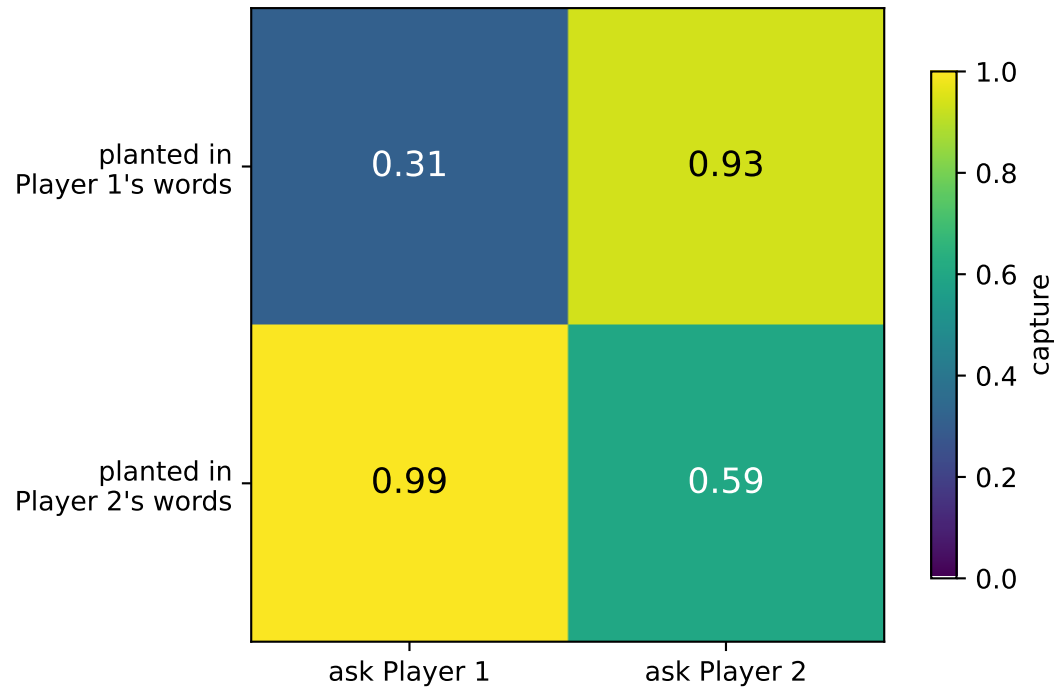
mech5: byte-identical history, only final request differs capture is HIGHER for the NON-owner → best-response matching
