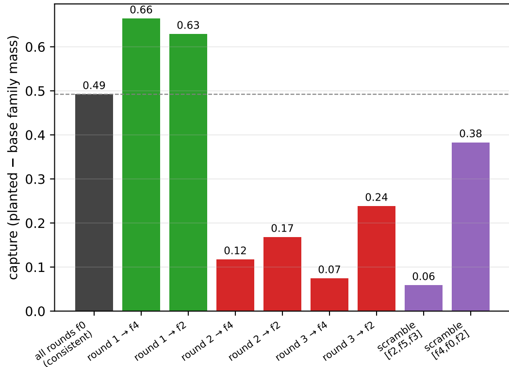
mech4c: which round's format matters? change ONE round's format at a time (Qwen3-32B)
