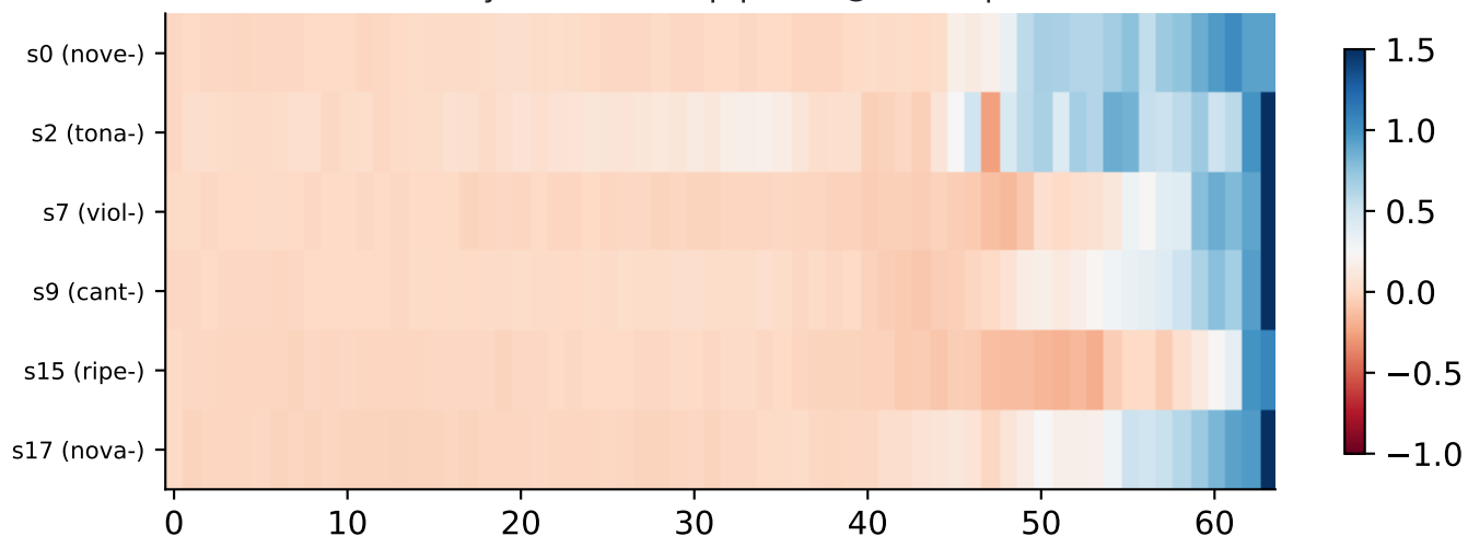
\Delta recovery, control→loop patch @ FINAL position
