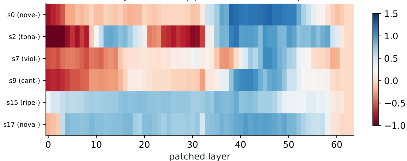
\Delta recovery, control→loop patch @ SEED-WORD spans
