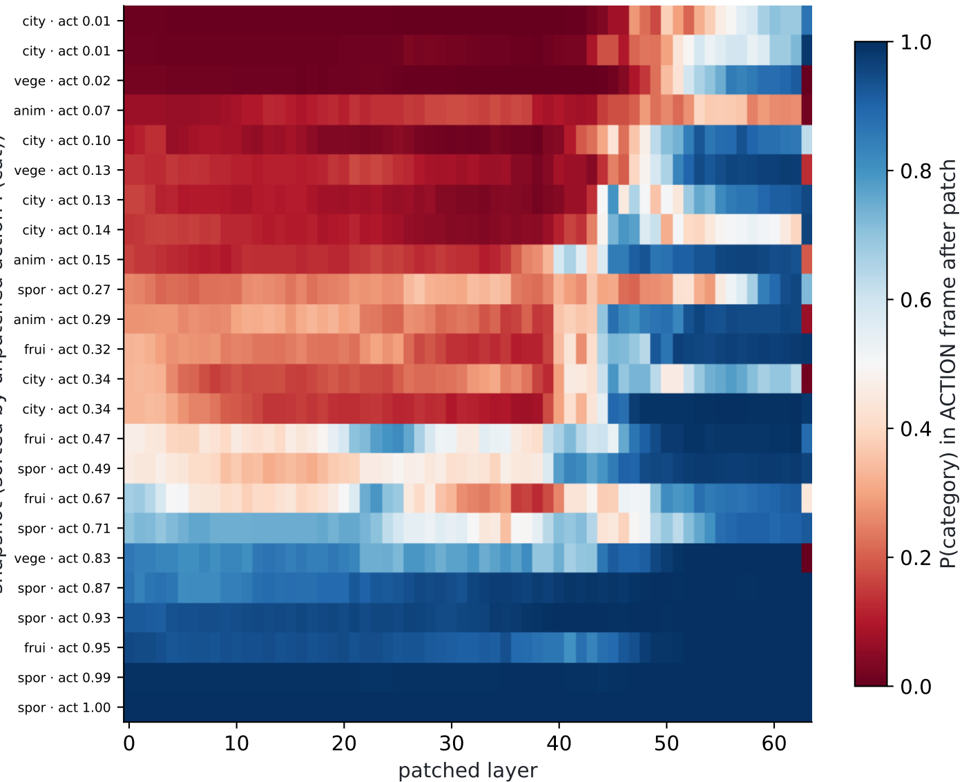
Per-snapshot patched action-frame category mass
