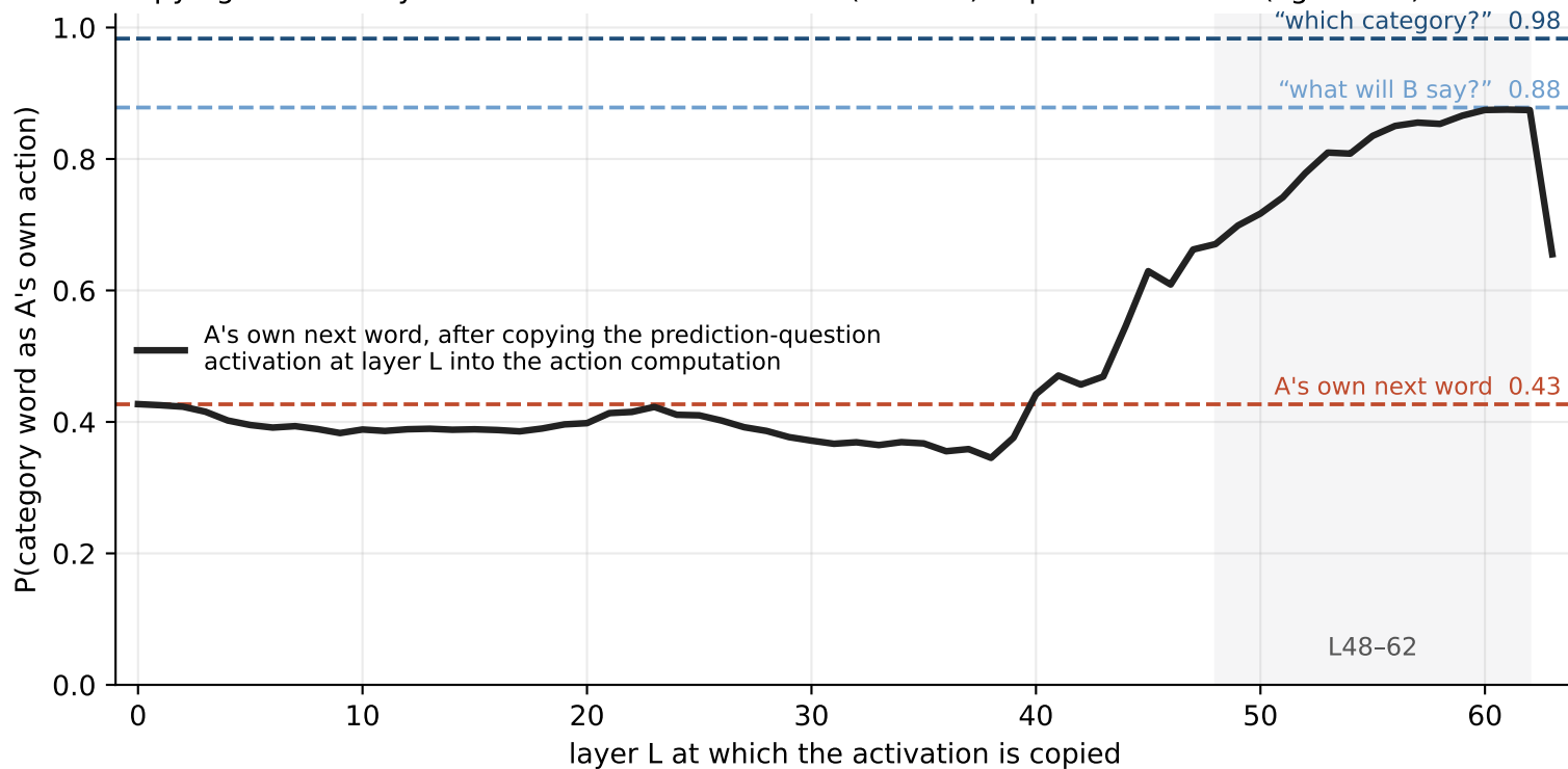
Copying one late layer's activation lifts the action (red line) to prediction level (light blue)
