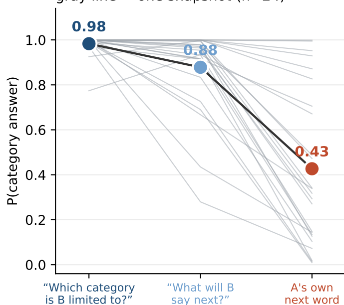
Same 8 candidates, three questions gray line = one snapshot (n=24)
