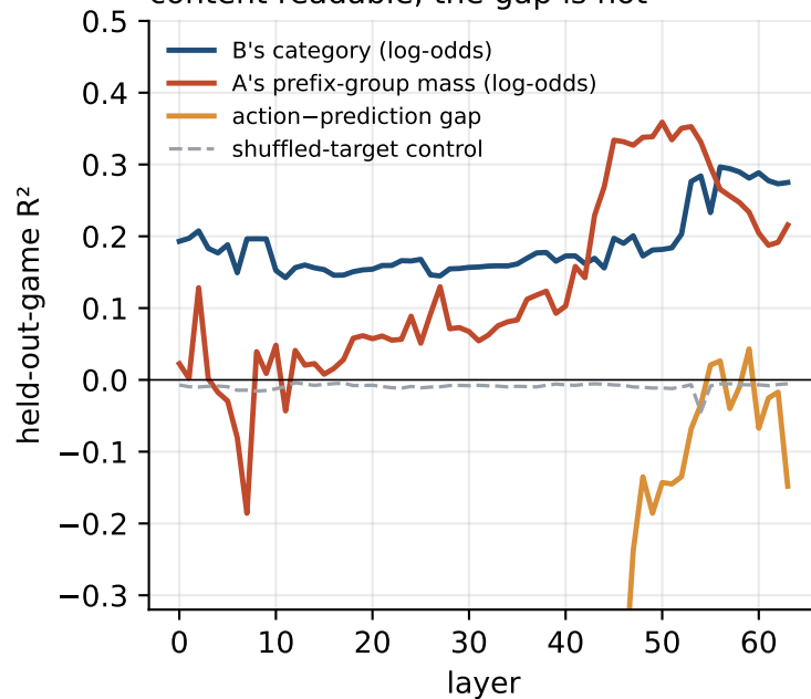
Linear probes on activations: content readable, the gap is not
