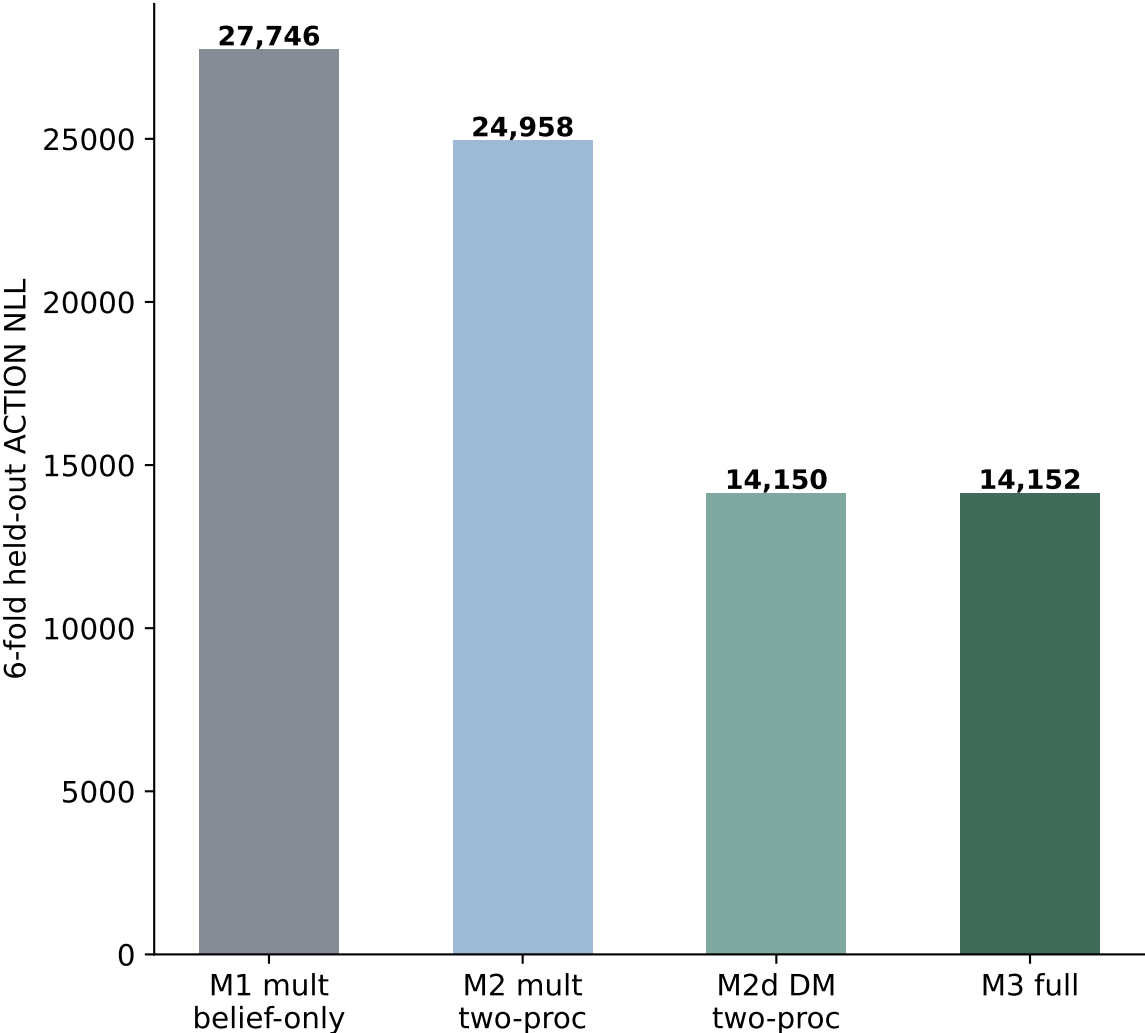
Model ladder (lower is better)
