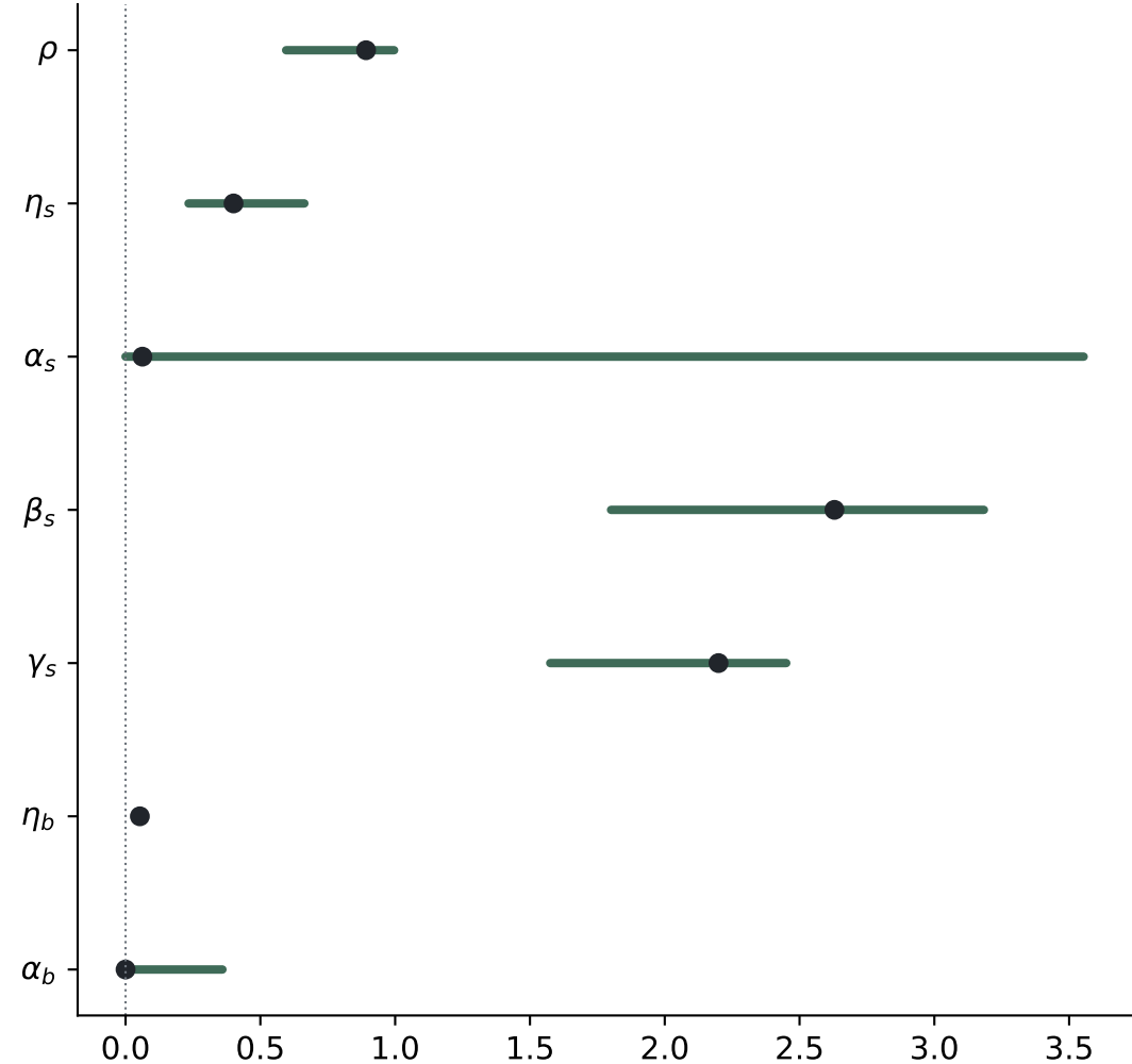
Game-level bootstrap 95% CIs (n=100)
