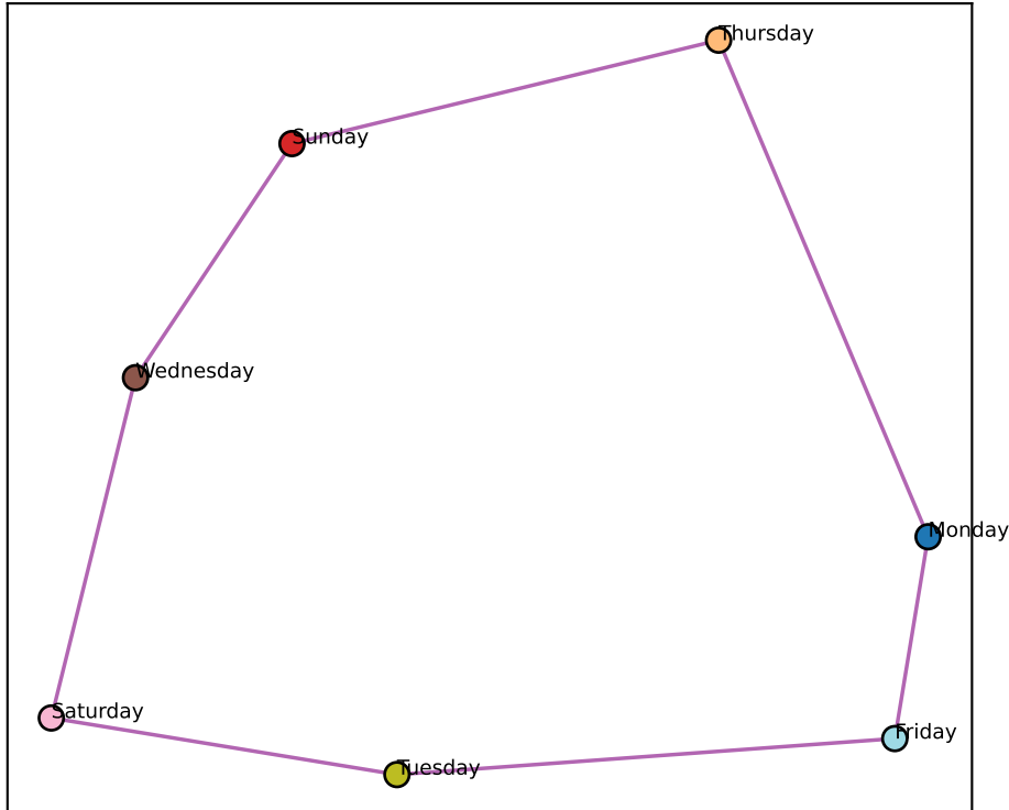
Llama L31 best-2D (node-mean) (ctx-RSA +0.87)
