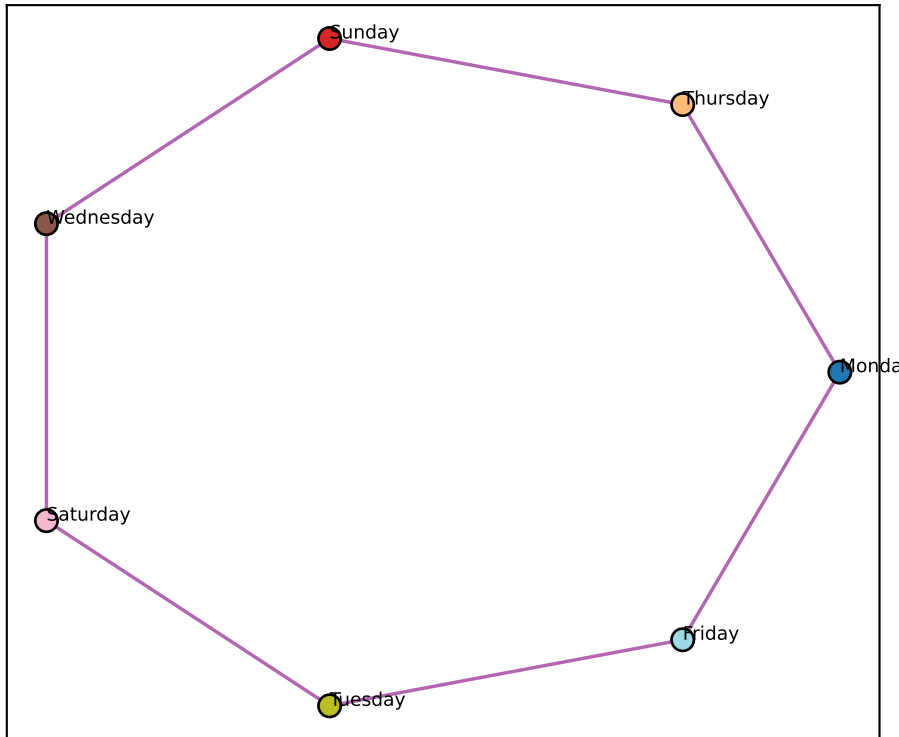
Llama L0 best-2D (node-mean) (ctx-RSA +0.85)
