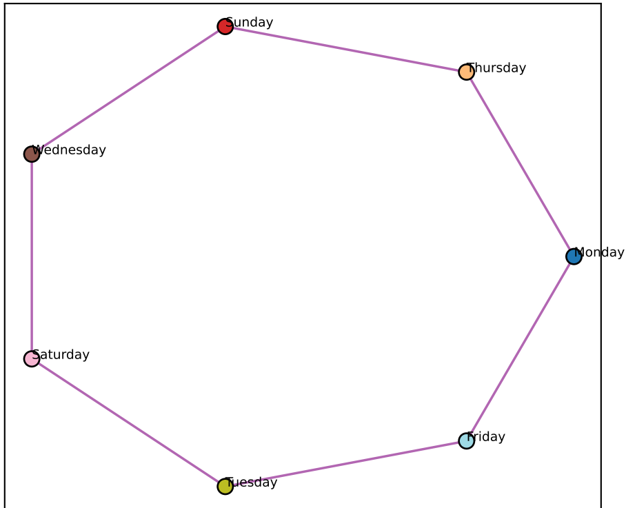
Llama L29 best-2D (node-mean) (ctx-RSA +0.89)
