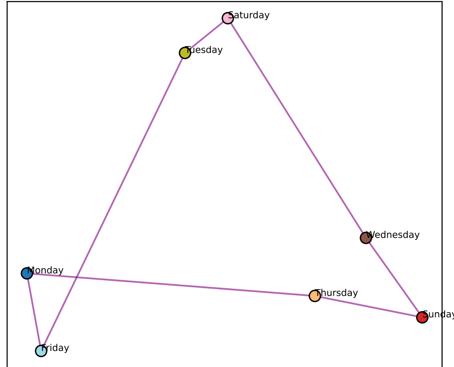
Gemma L11 best-2D (node-mean) (ctx-RSA +0.89)
