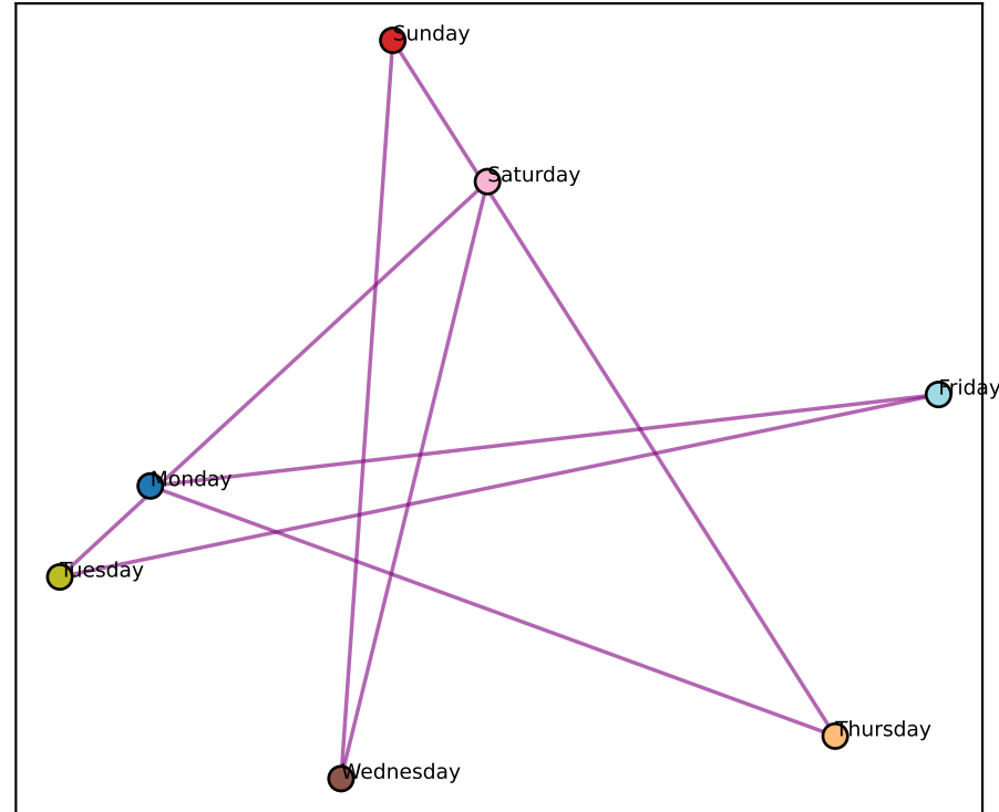
Gemma L21 best-2D (node-mean) (ctx-RSA +0.91)
