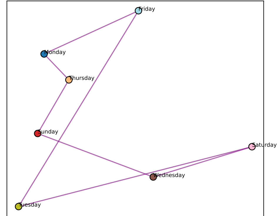
Qwen L3 best-2D (node-mean) (ctx-RSA +0.88)
