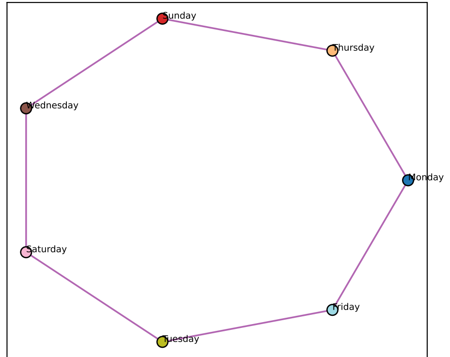
Gemma L29 best-2D (node-mean) (ctx-RSA +0.91)
