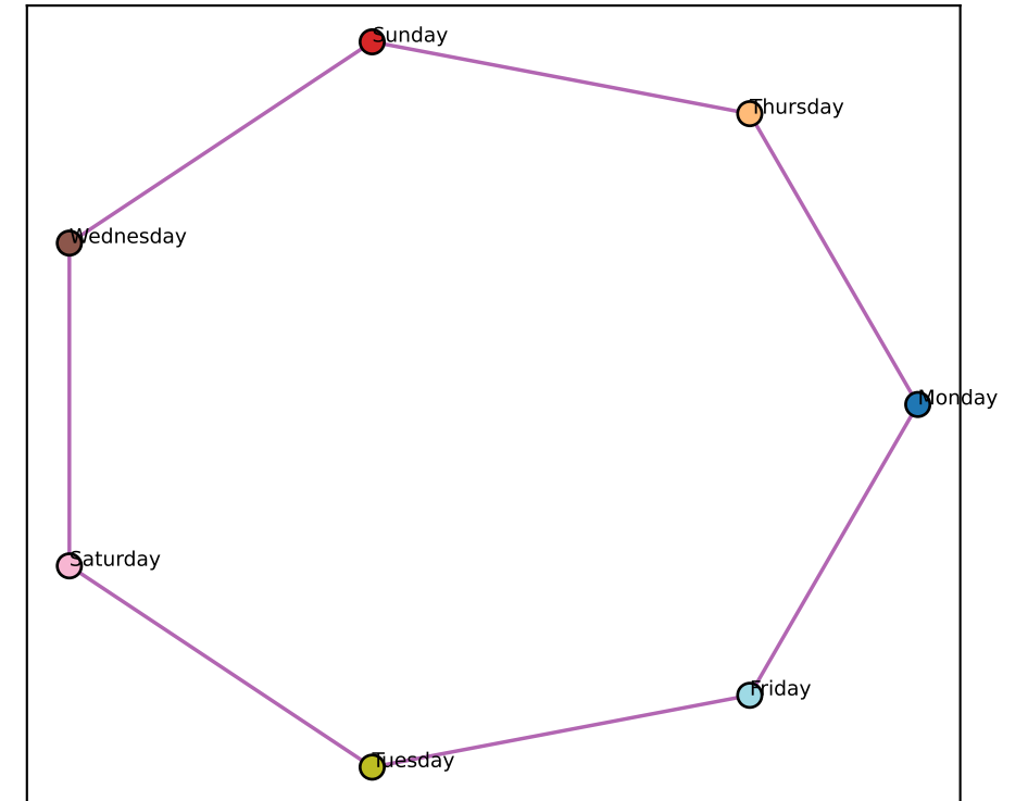
Qwen L11 best-2D (node-mean) (ctx-RSA +0.93)
