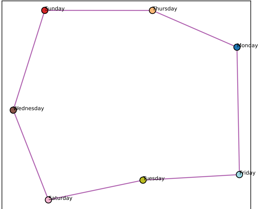
Llama L17 best-2D (node-mean) (ctx-RSA +0.94)
