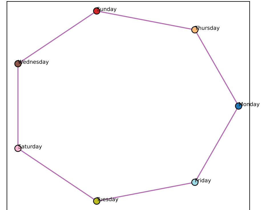
Qwen L14 best-2D (node-mean) (ctx-RSA +0.90)
