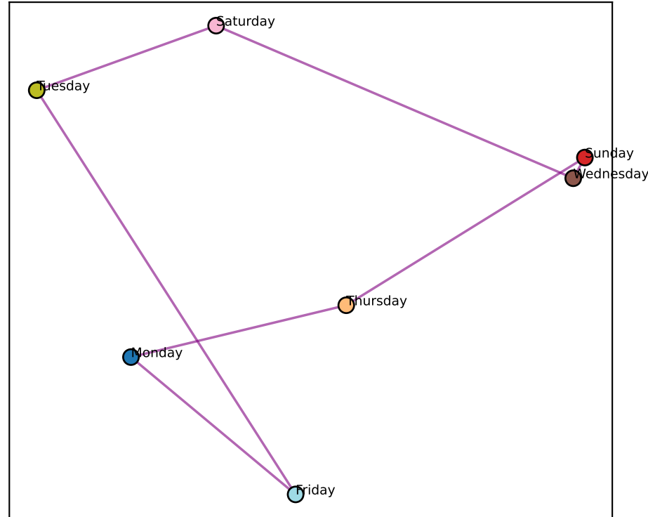
Gemma L13 best-2D (node-mean) (ctx-RSA +0.87)
