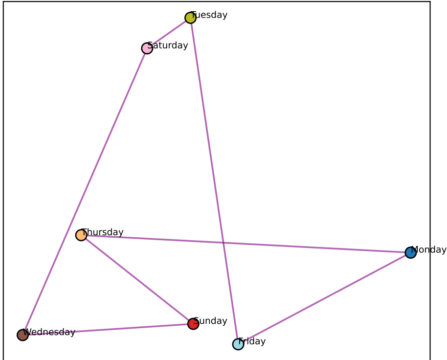
Llama L8 best-2D (node-mean) (ctx-RSA +0.91)
