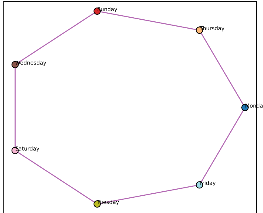
Gemma L35 best-2D (node-mean) (ctx-RSA +0.90)
