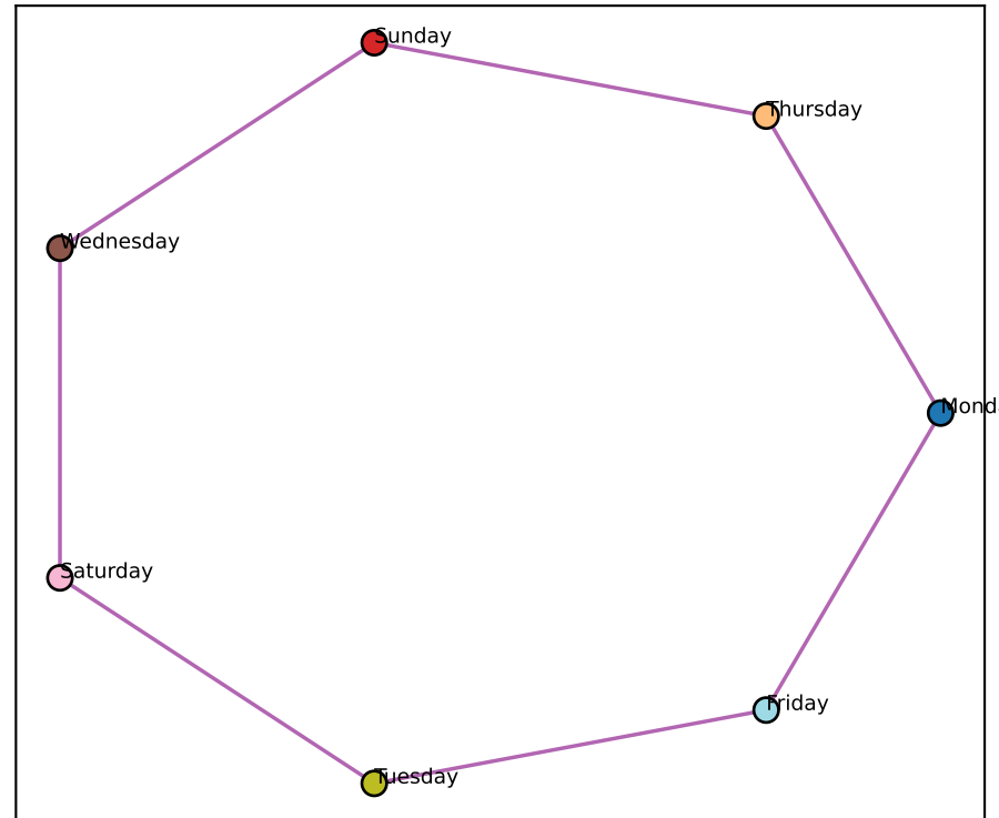
Gemma L22 best-2D (node-mean) (ctx-RSA +0.90)
