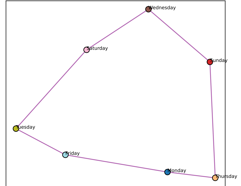
Qwen L33 best-2D (node-mean) (ctx-RSA +0.90)
