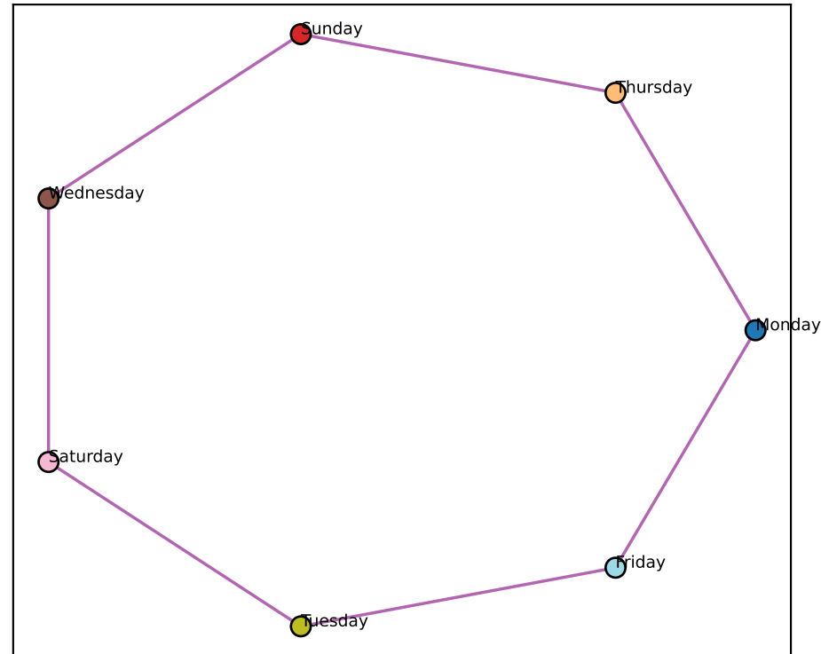
Gemma L8 best-2D (node-mean) (ctx-RSA +0.90)
