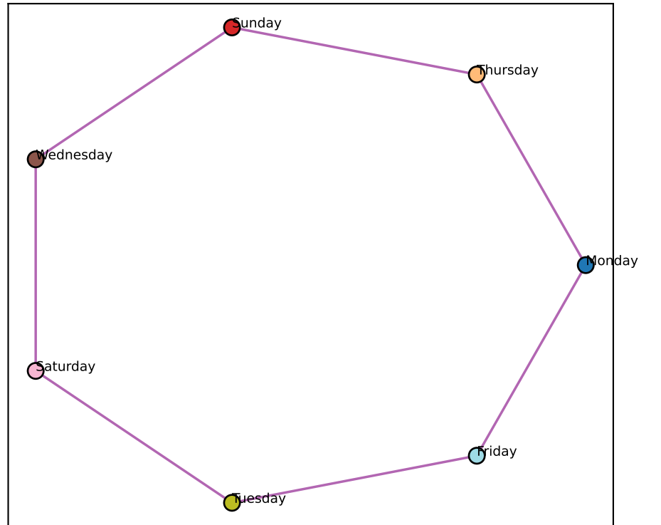
Gemma L18 best-2D (node-mean) (ctx-RSA +0.86)
