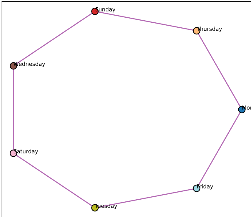
Llama L7 best-2D (node-mean) (ctx-RSA +0.85)
