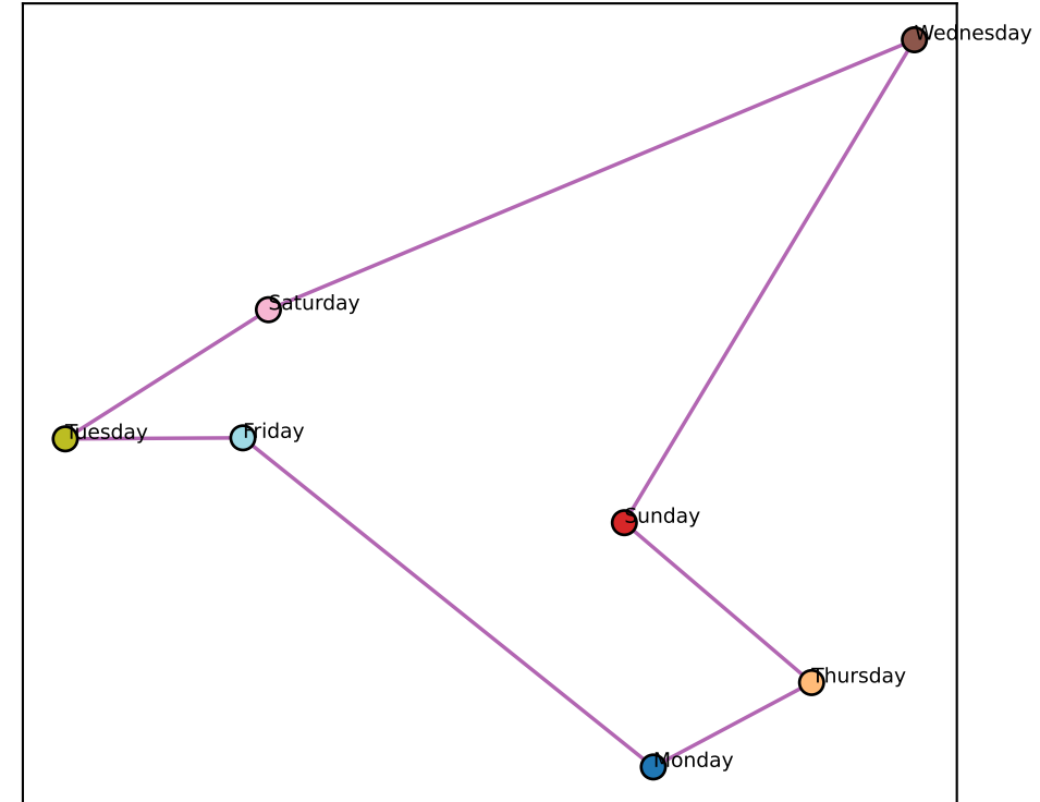
Qwen L27 best-2D (node-mean) (ctx-RSA +0.86)
