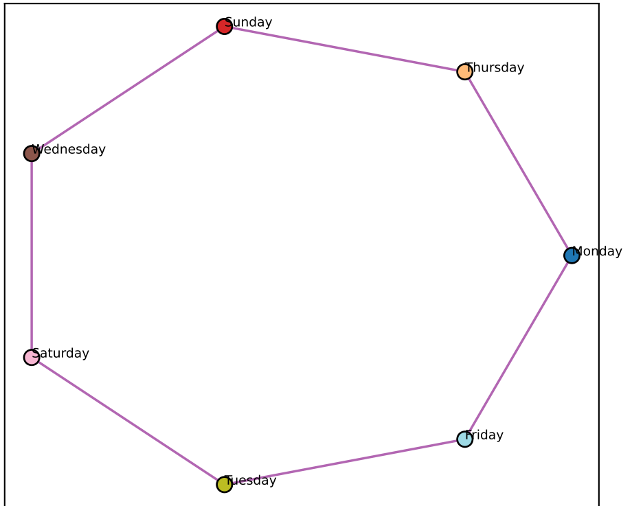
Llama L27 best-2D (node-mean) (ctx-RSA +0.91)
