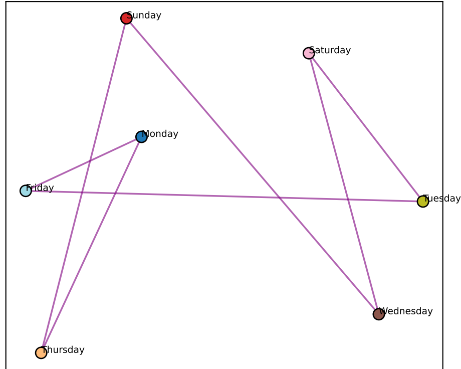
Gemma L25 best-2D (node-mean) (ctx-RSA +0.85)
