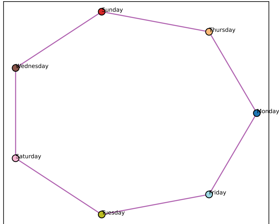
Gemma L26 best-2D (node-mean) (ctx-RSA +0.86)
