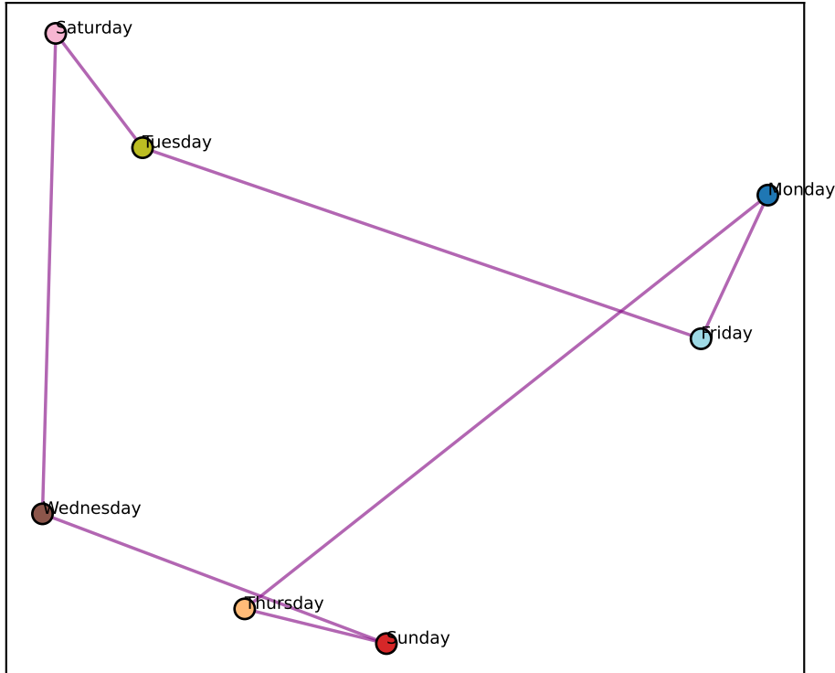
Llama L2 best-2D (node-mean) (ctx-RSA +0.90)
