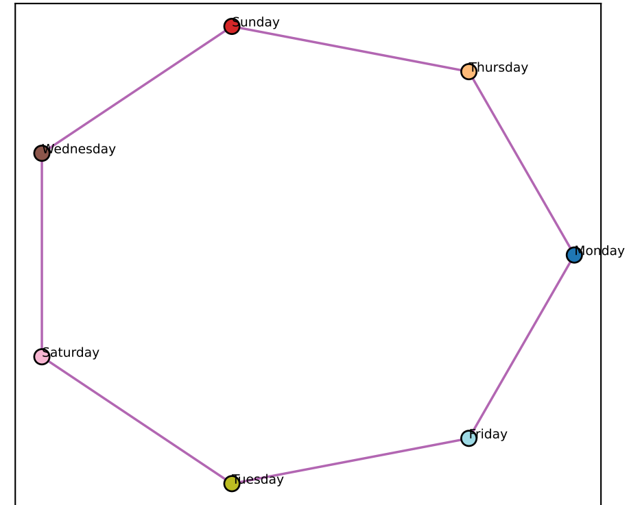
Qwen L8 best-2D (node-mean) (ctx-RSA +0.89)
