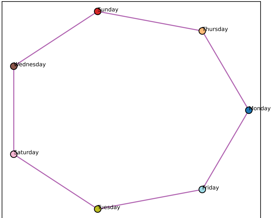
Llama L19 best-2D (node-mean) (ctx-RSA +0.85)
