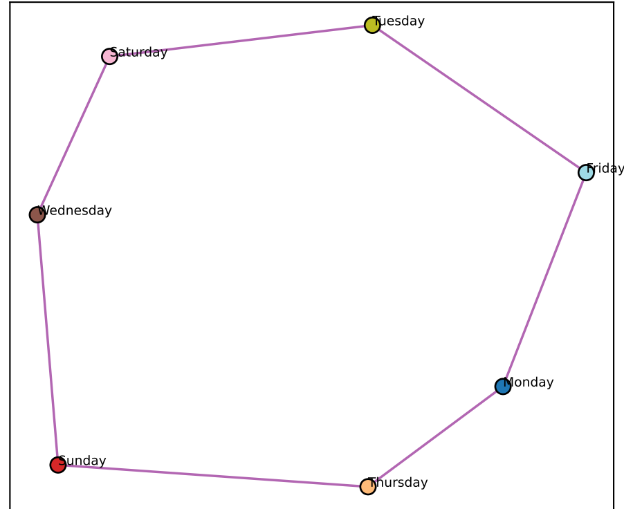
Gemma L28 best-2D (node-mean) (ctx-RSA +0.91)
