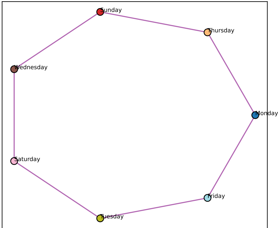
Llama L24 best-2D (node-mean) (ctx-RSA +0.88)
