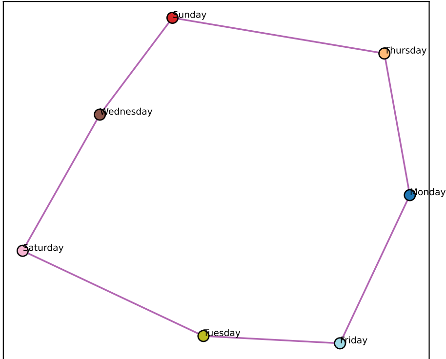
Llama L25 best-2D (node-mean) (ctx-RSA +0.86)
