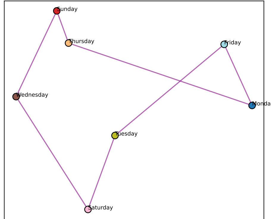
Gemma L0 best-2D (node-mean) (ctx-RSA +0.87)
