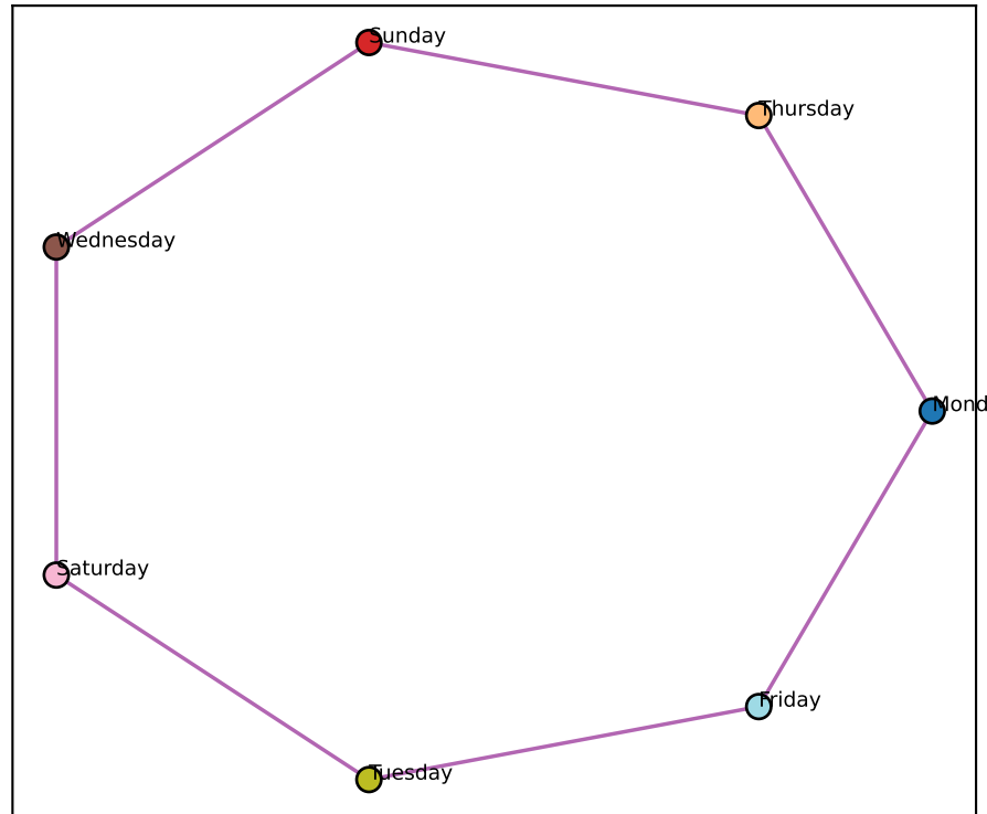
Gemma L15 best-2D (node-mean) (ctx-RSA +0.91)
