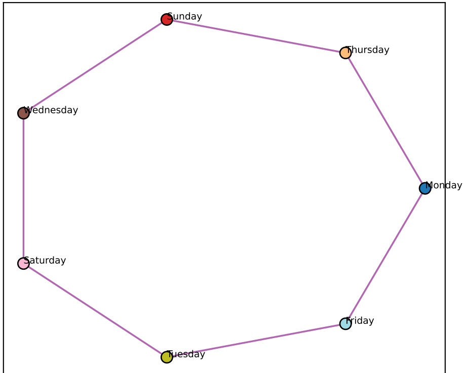
Llama L20 best-2D (node-mean) (ctx-RSA +0.91)
