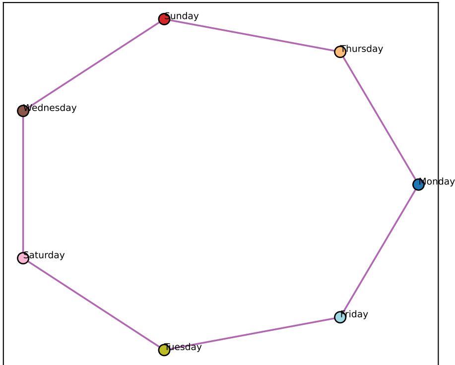
Llama L4 best-2D (node-mean) (ctx-RSA +0.89)
