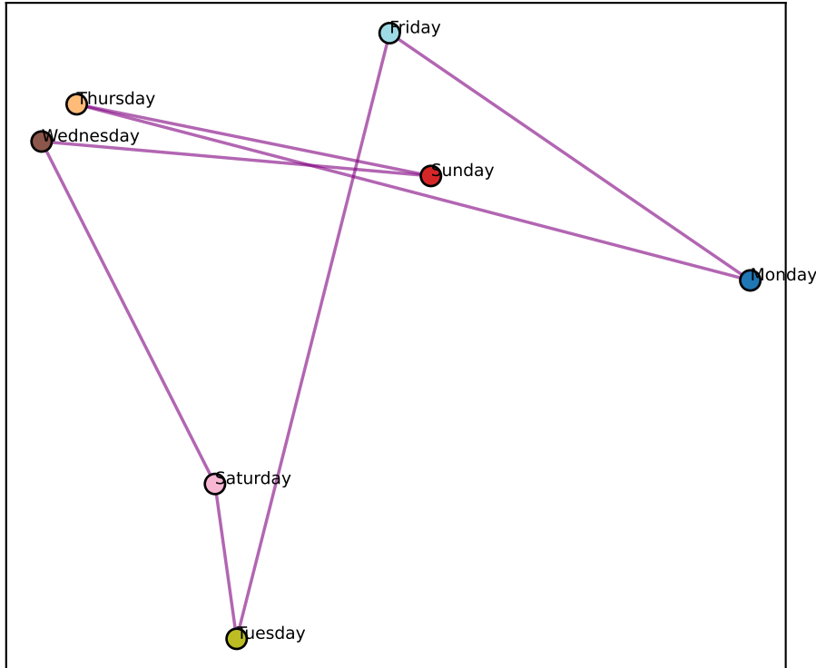
Llama L10 best-2D (node-mean) (ctx-RSA +0.82)
