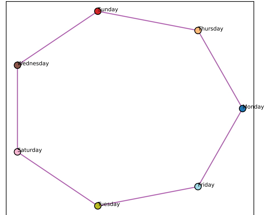
Qwen L15 best-2D (node-mean) (ctx-RSA +0.91)
