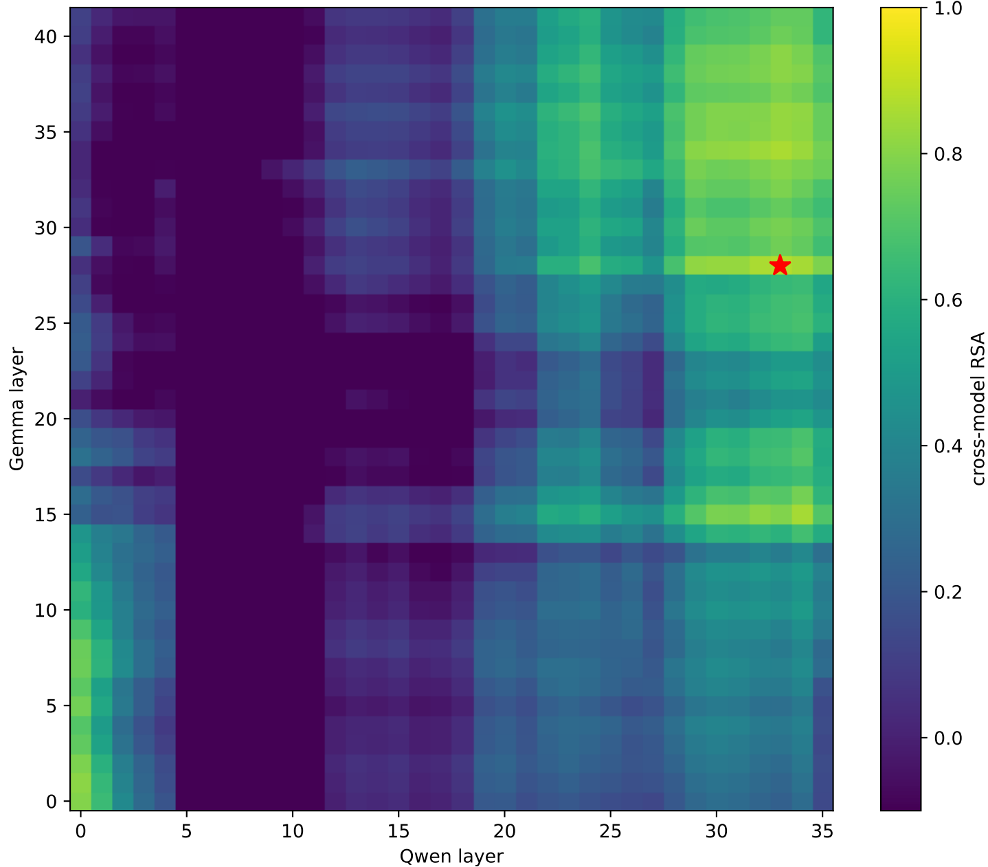
days: Gemma vs Qwen cross-model RSA (max 0.87 @ Gemma L28 / Qwen L33)
