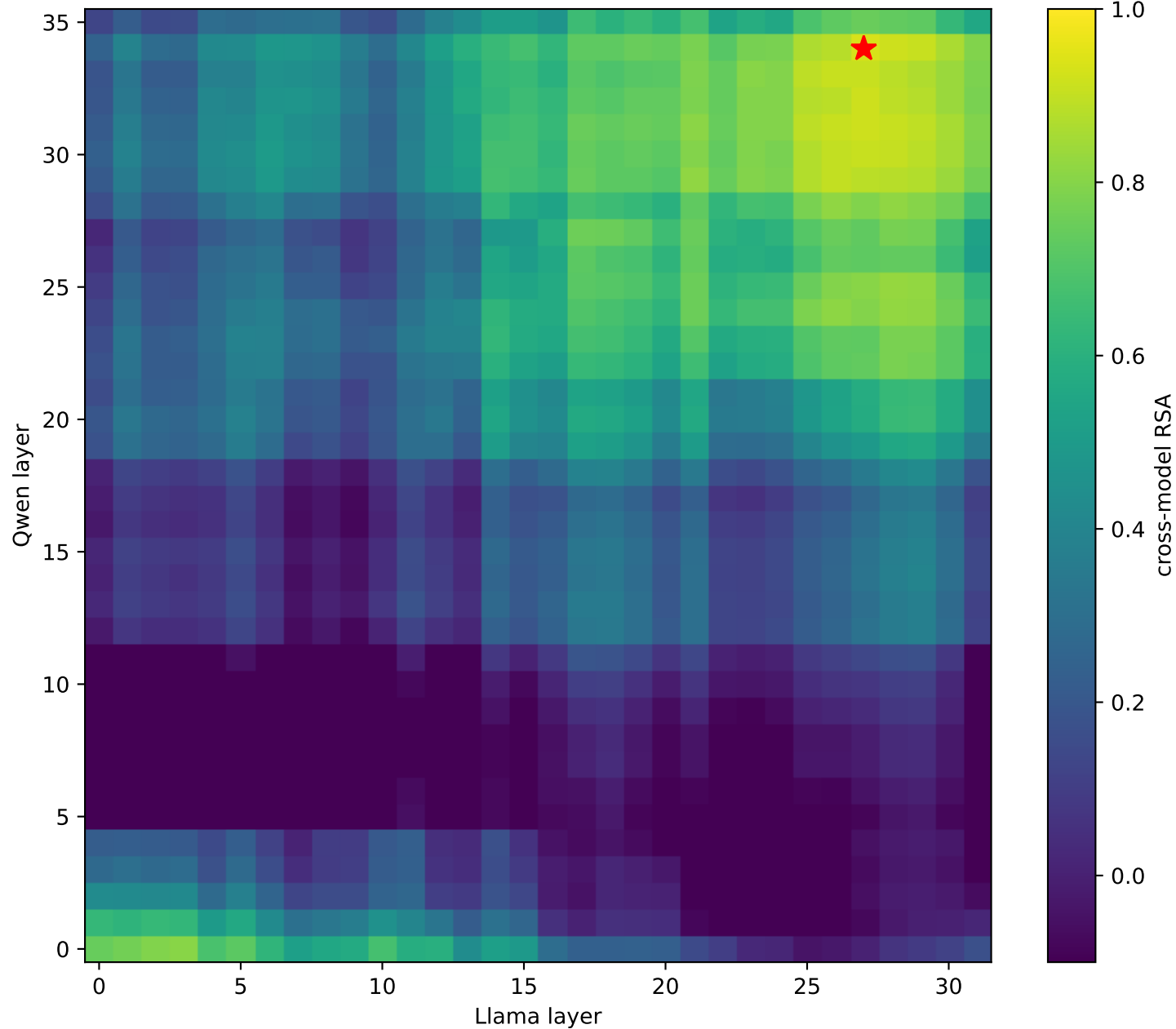
days: Qwen vs Llama cross-model RSA (max 0.93 @ Qwen L34 / Llama L27)
