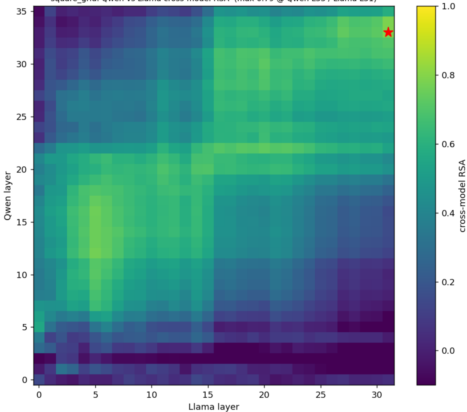
square_grid: Qwen vs Llama cross-model RSA (max 0.79 @ Qwen L33 / Llama L31)
