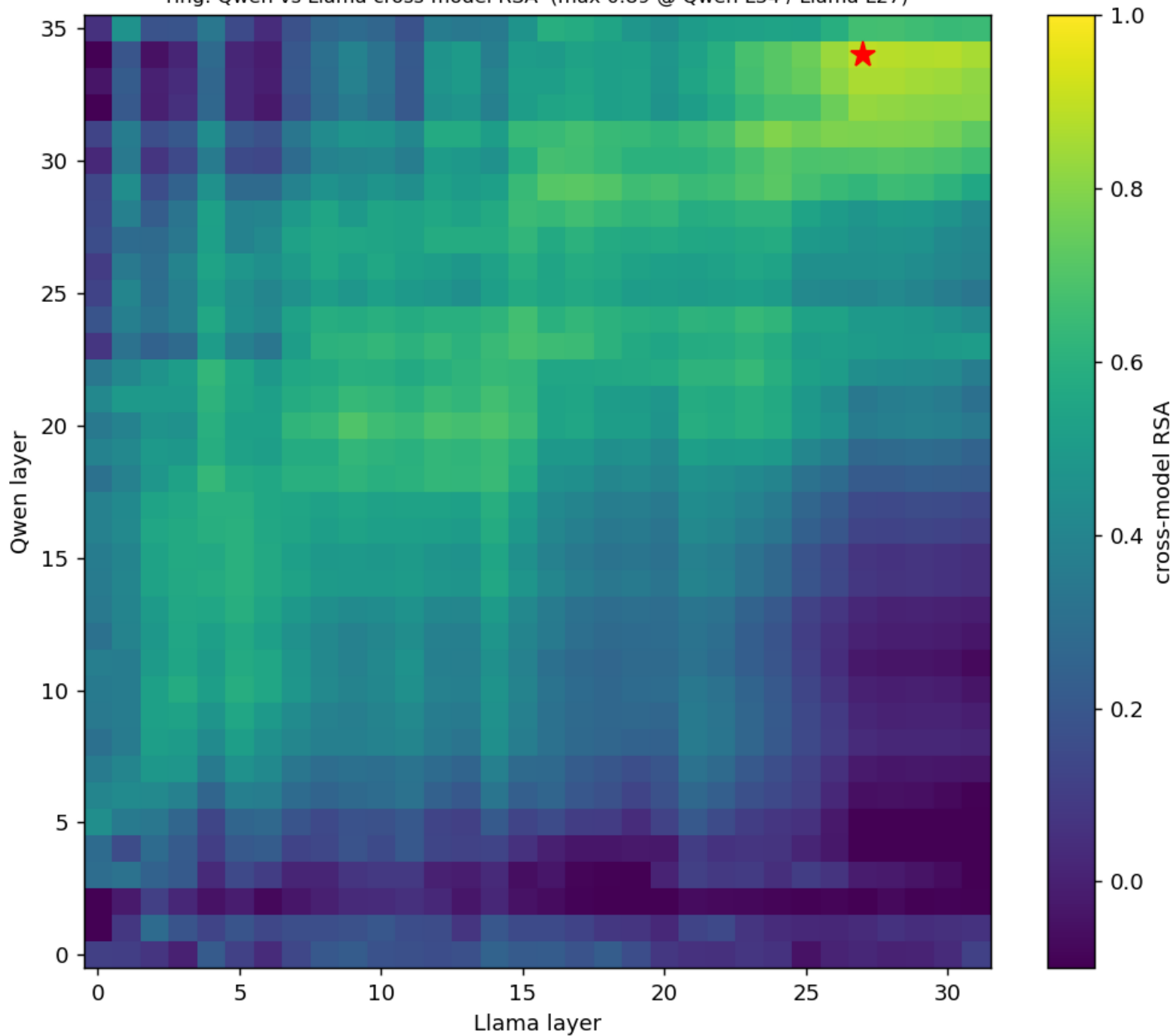
ring: Qwen vs Llama cross-model RSA (max 0.89 @ Qwen L34 / Llama L27)
