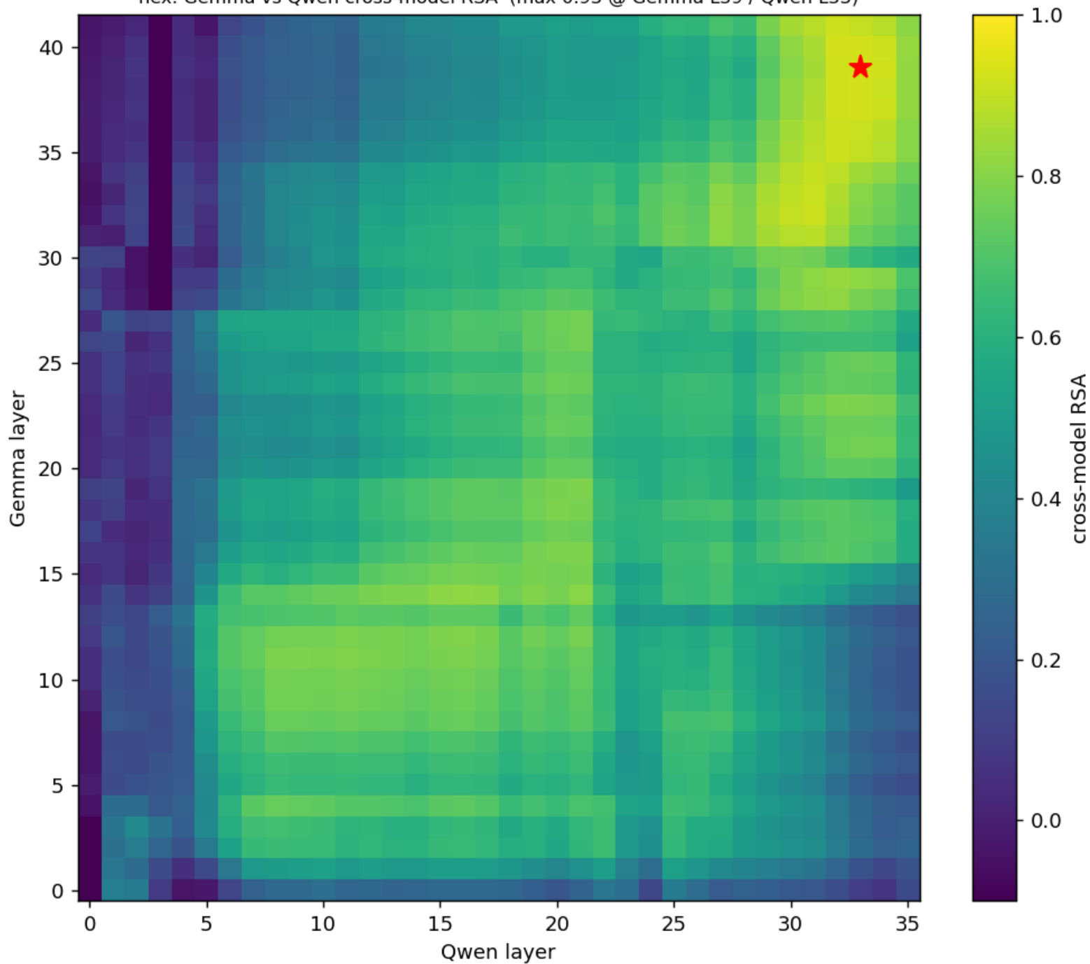
hex: Gemma vs Qwen cross-model RSA (max 0.93 @ Gemma L39 / Qwen L33)
