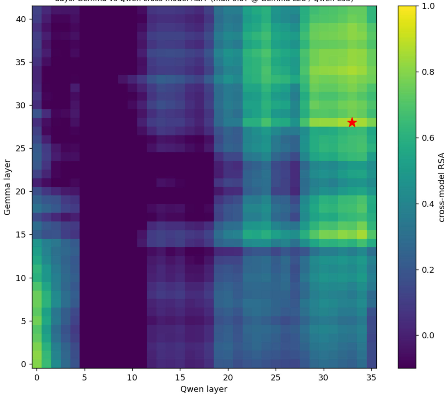
days: Gemma vs Qwen cross-model RSA (max 0.87 @ Gemma L28 / Qwen L33)
