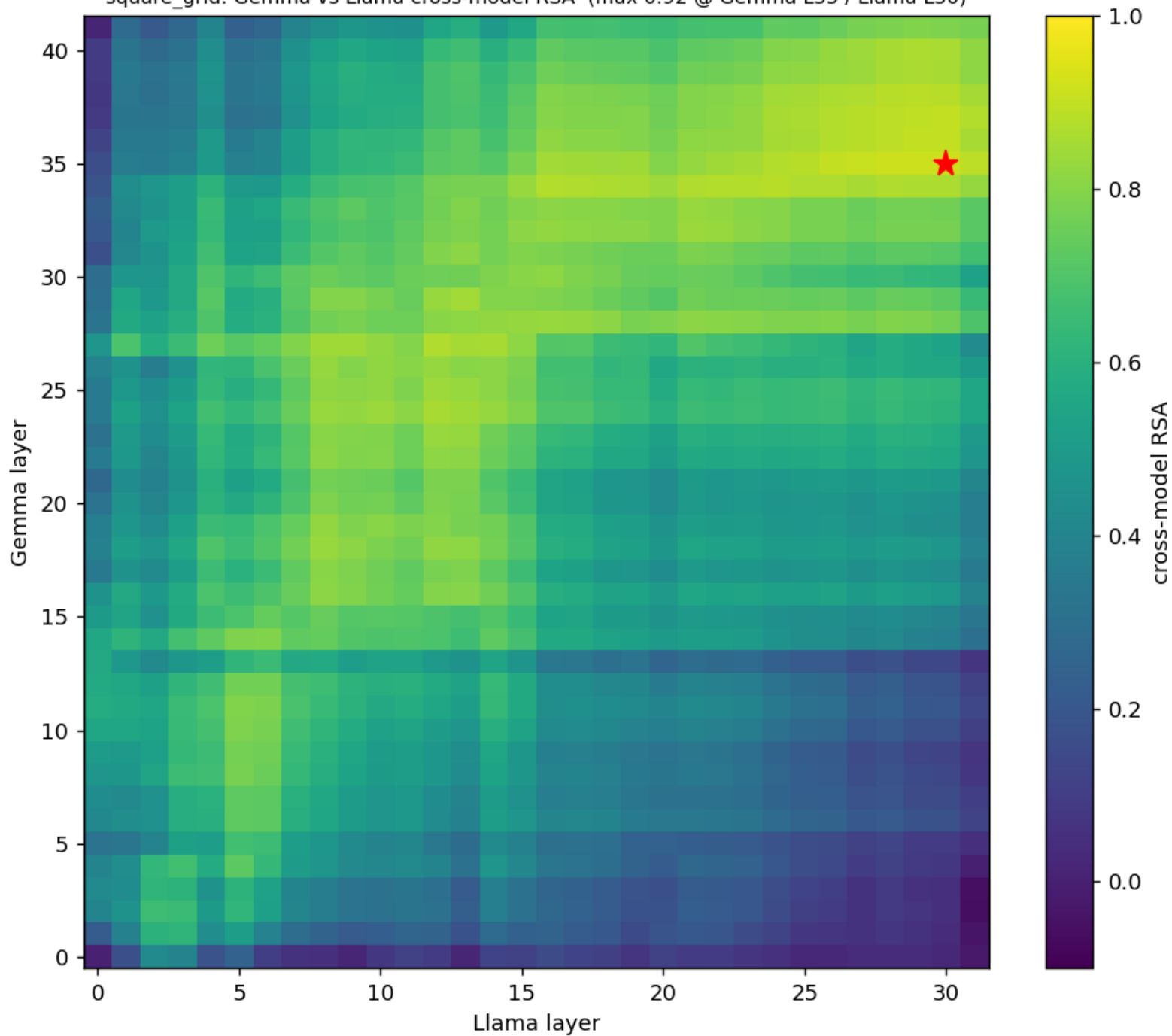
square_grid: Gemma vs Llama cross-model RSA (max 0.92 @ Gemma L35 / Llama L30)
