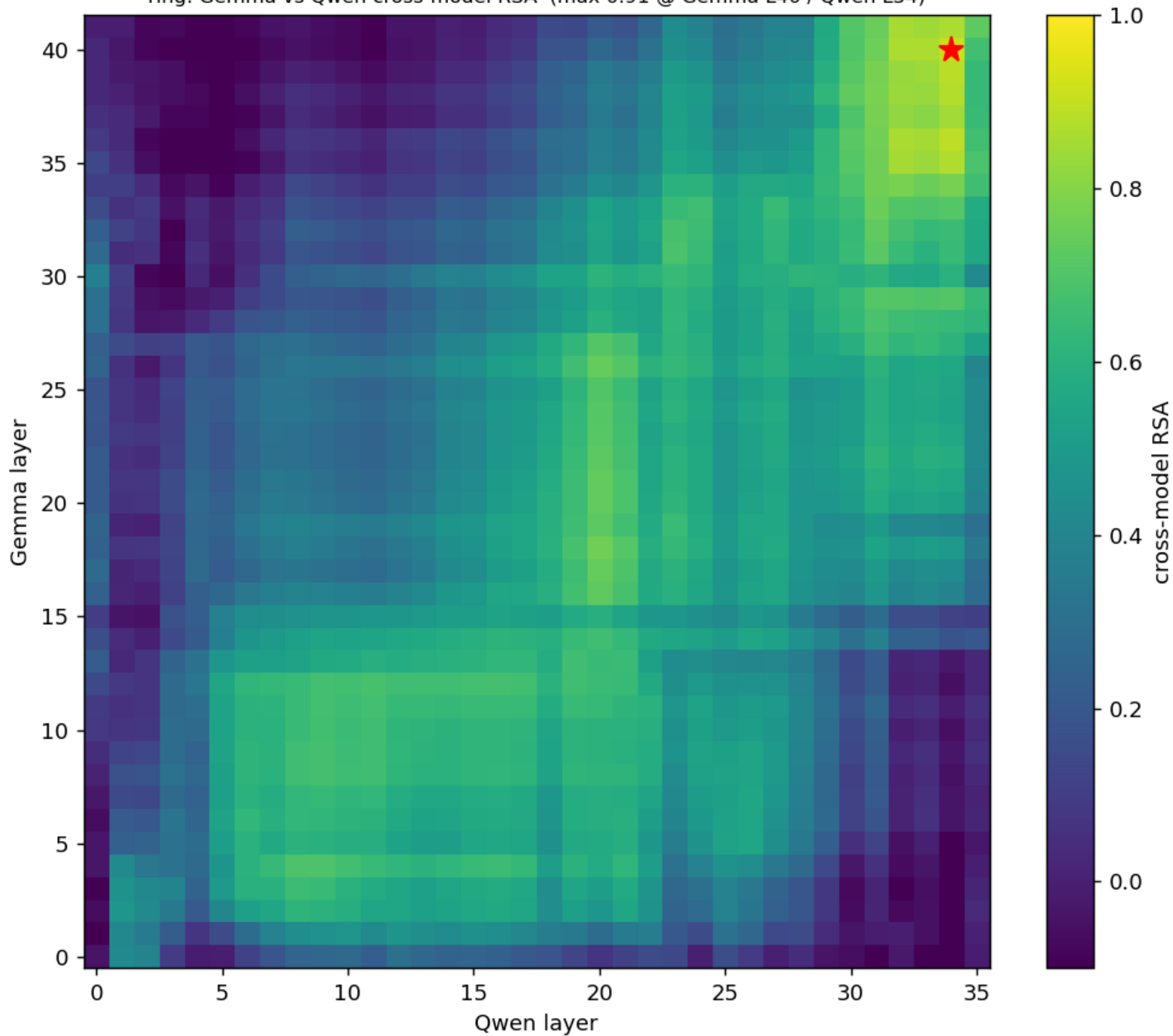
ring: Gemma vs Qwen cross-model RSA (max 0.91 @ Gemma L40 / Qwen L34)
