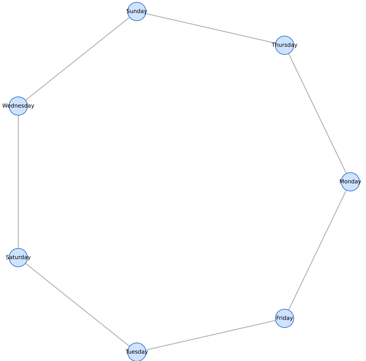
Graph: 7 nodes
