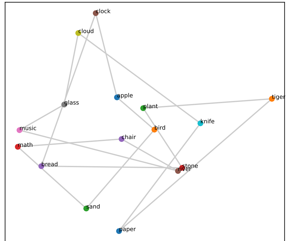
Qwen L10 (RSA=-0.06)
